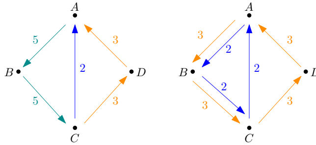
Fig. 2: The graph on the left depicts a circulation. The weight of each edge is the transaction amount to send along the edge. The cycles in the graph on the right is a sign consistent decomposition of the the circulation.
