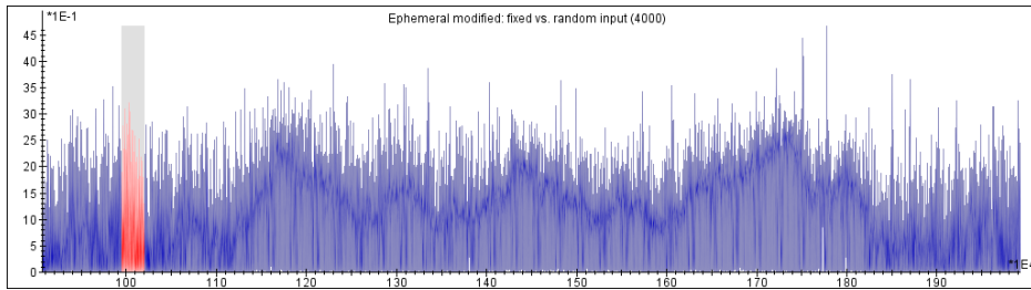
Figure 9: Modified ephemeral implementation TVLA: (0.9ms-2.0ms): fixed vs random point.
