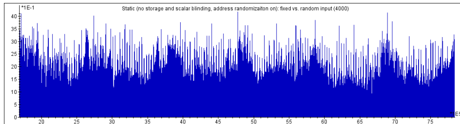
Figure 13: Static impl. with blindings turned off and the address rand. turned on TVLA (1.7-7.8ms), aligned at 1.65ms: fixed vs random scalar.
