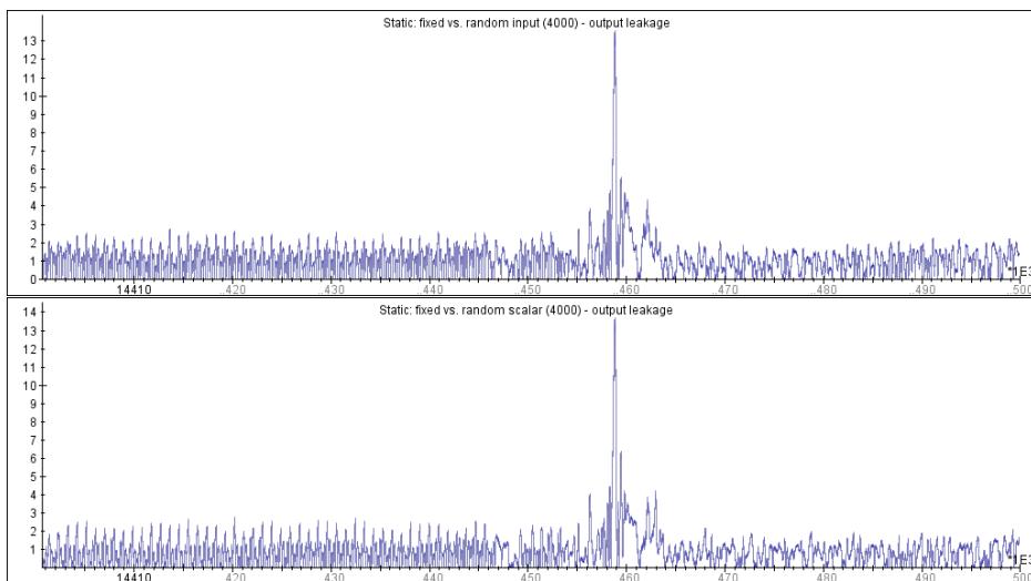
Figure 11: Static implementation TVLA (14.4-14.5ms), aligned at 13.0ms: fixed vs random point (top) and fixed vs random scalar (bottom).
