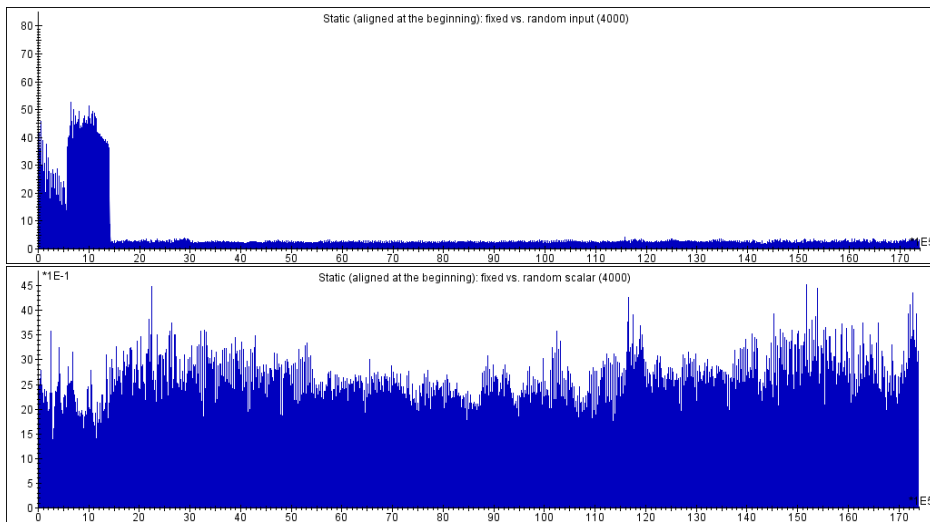
Figure 10: Static implementation TVLA: fixed vs random point (top) and fixed vs random scalar (bottom).
