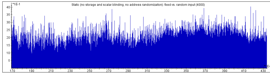
Figure 12: Static impl. with blindings and address randomization disabled TVLA (1.7-4.3ms), aligned at 1.65ms: fixed vs random point.
