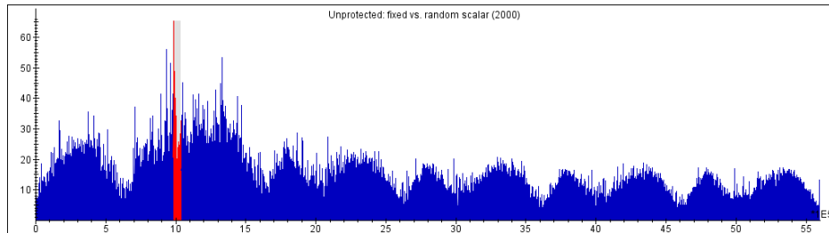
Figure 8: Unprotected implementation TVLA: fixed vs random scalar.
