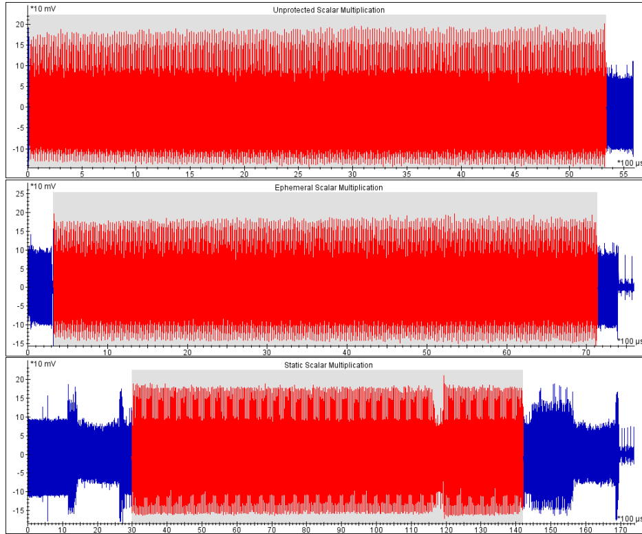
Figure 7: Power profiles of unprotected (top), ephemeral (middle), and static (bottom) implementations.
