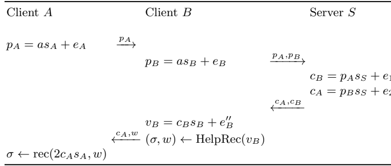
Fig. 2. A brief description of the data transmission to realize key exchange.
