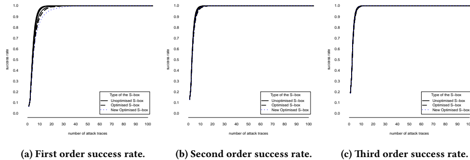
Figure 2: Success rates (different orders) of correlation power analysis on 4 × 4 S-boxes as a function of the number of attack traces. The standard deviation of the noise equals \sigma = 0.5 . The S-boxes have nonlinearity equal to N_F = 4 and differential uniformity equal to \delta_F = 4 .
