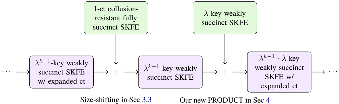
Figure 2: An illustration of our iteration technique, in which our size-shifting procedure is sandwiched. For k -th iteration, first, we apply the size-shifting procedure to a \lambda^{k-1} -key weakly succinct SKFE scheme with expanded ciphertexts incurred by nested-ciphertext-embedding (the result of (k-1) -th iteration). Second, we apply our new PRODUCT construction to increase the number of issuable keys.
