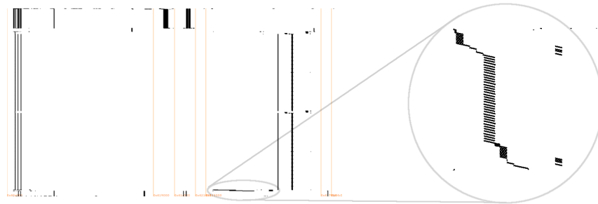
Fig. 9. Visualization of the instructions in a software execution trace of the Karroumi WB-AES implementation by Klinec, with a zoom on the core of the white-box.
