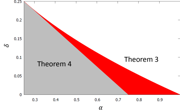
Figure 2: Comparison between our attack (Theorem 3) and the attack of Lu et al. (Theorem 4) [LZPL15].
