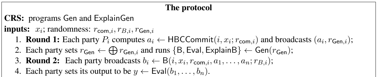
Figure 2: MPC protocol.
