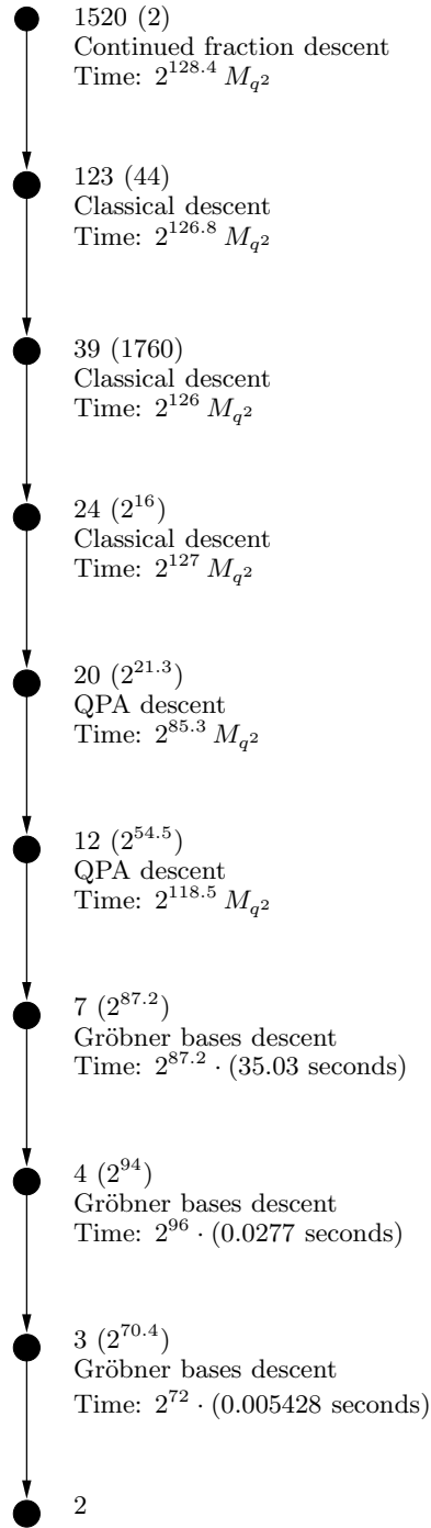
FIGURE 2. A typical path of the descent tree for computing an individual logarithm in \mathbb{F}_{2^{24-3041}} ( q = 2^{12} ). The numbers in parentheses next to each node are the expected number of nodes at that level. ‘Time’ is the expected time to generate all nodes at a level.
