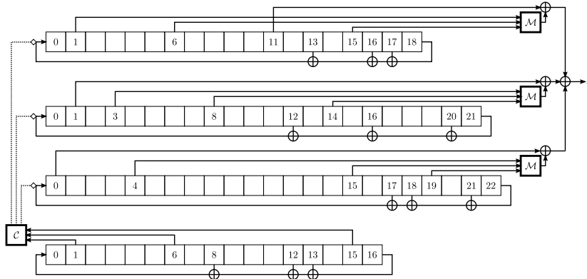
Figure 2: The A5-GMR-1 cipher
