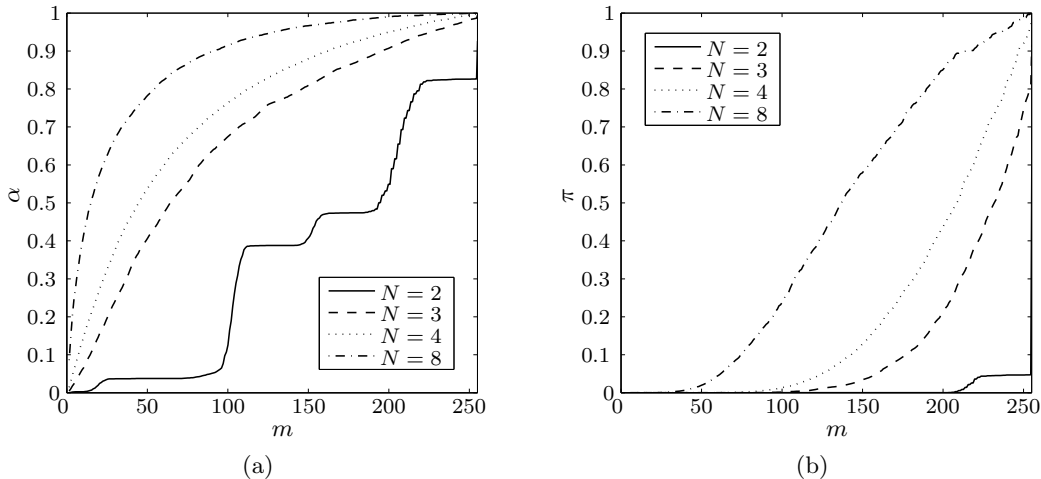
Fig. 4. Empirical dependency of \alpha and \pi upon m for different numbers of traces N
