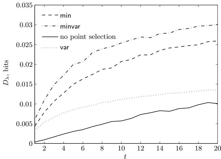
Fig. 8. Collision detection: effect of dimension reduction
