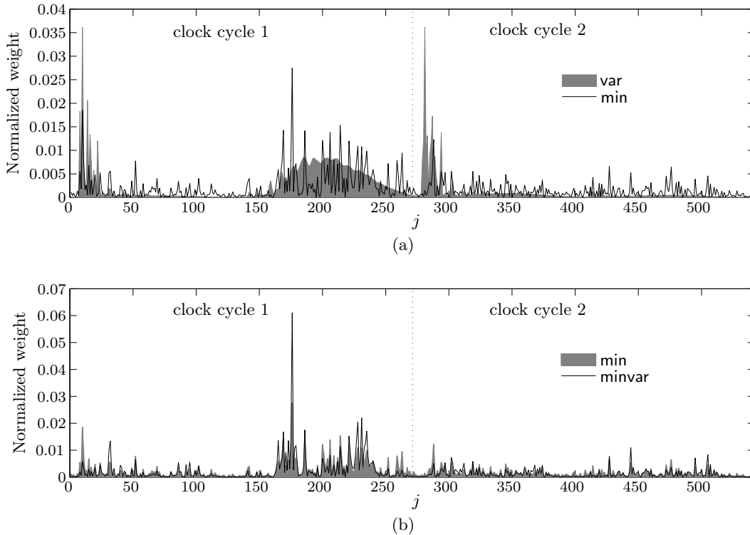
Fig. 6. Informative points for DPA vs. signal difference (a), and the effect of weighting signal difference with noise variance (b)
