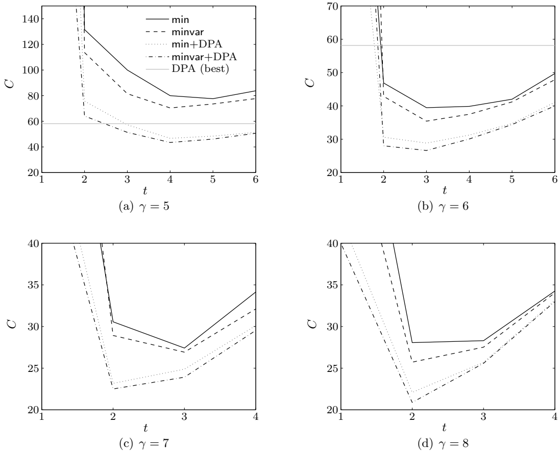
Fig. 9. Attack efficiency C = C_{\text{online}}/\pi in practice, against averaging t , for different numbers \gamma of inputs
