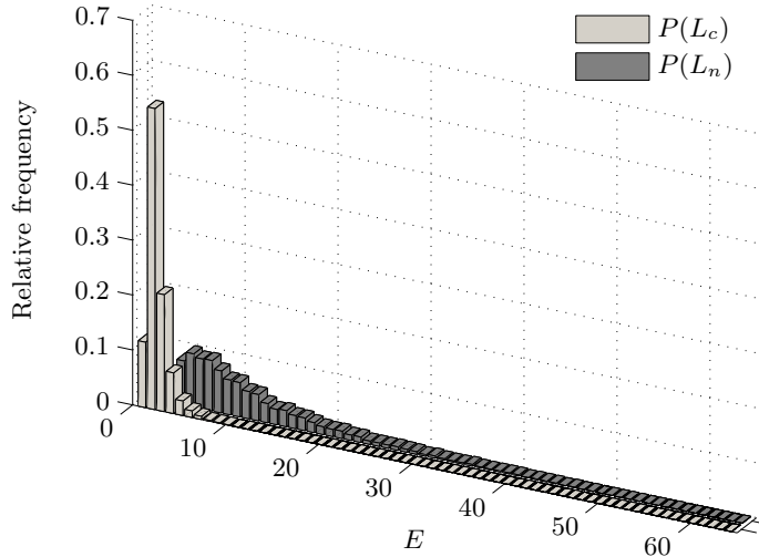
Fig. 7. Empirical distributions for P(L_c) and P(L_n)
