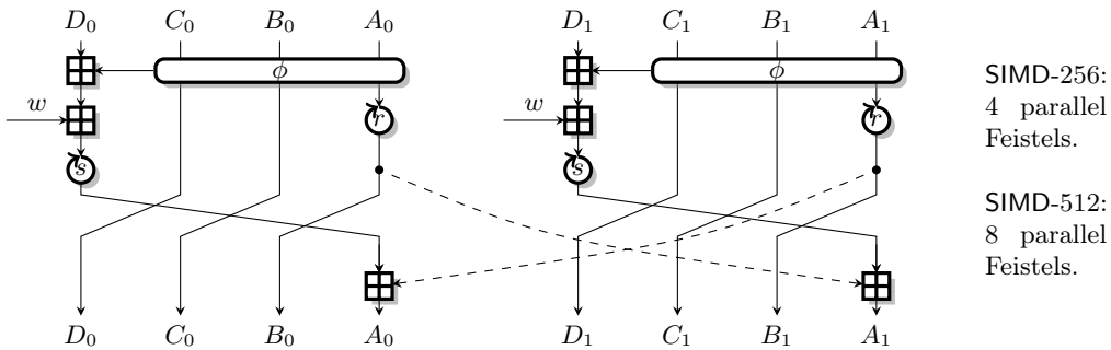
Fig. 2. SIMD compression rounds.
