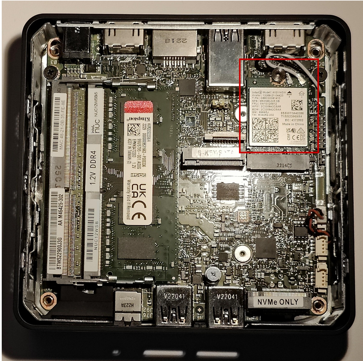
Fig. 1: The location of the wireless card within the NUC12
