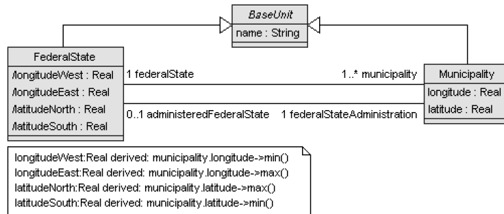
Fig. 7. Derived properties employing aggregate function in OCL
