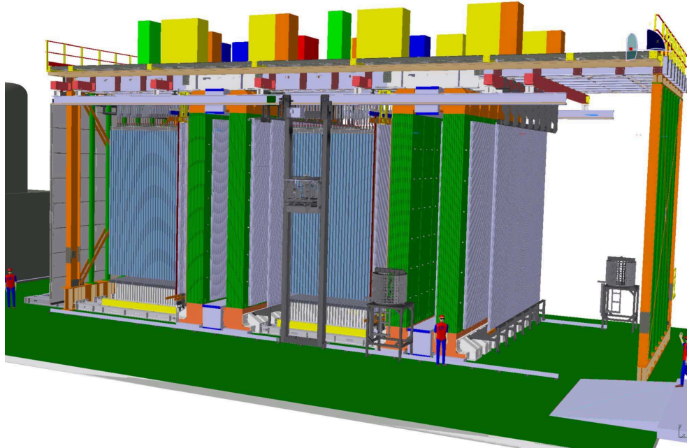
Figure 1: Schematic drawing of the OPERA detector at LNGS.
