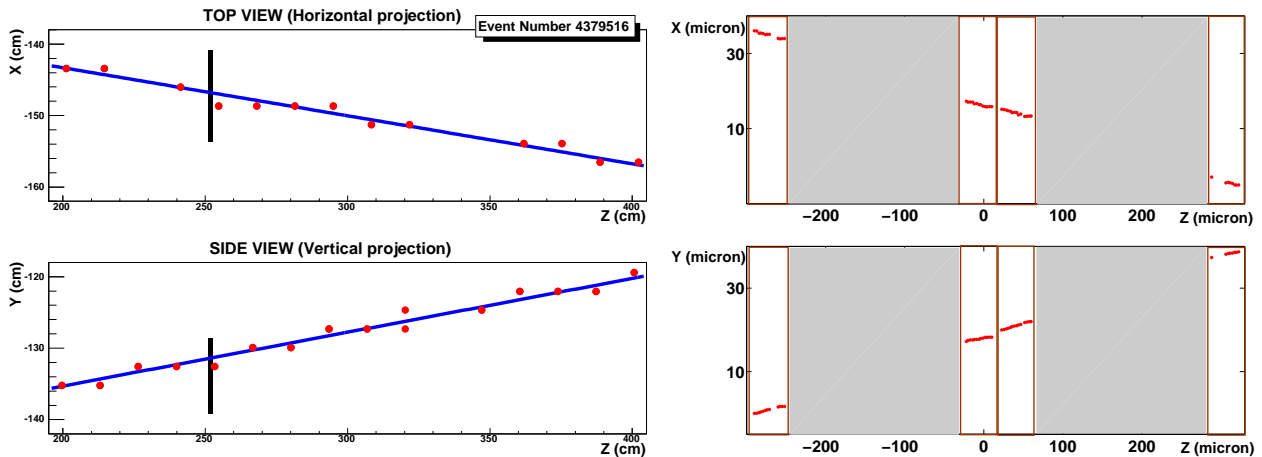
Figure 7: Left: display of one event with the muon passing through the CS detector plane. Only hits of the electronic detectors close to the CS plane are shown; the vertical segment indicates the position of the CS doublet intercepted by the track. Right: display of the corresponding 4 micro-tracks reconstructed in the CS doublet.
