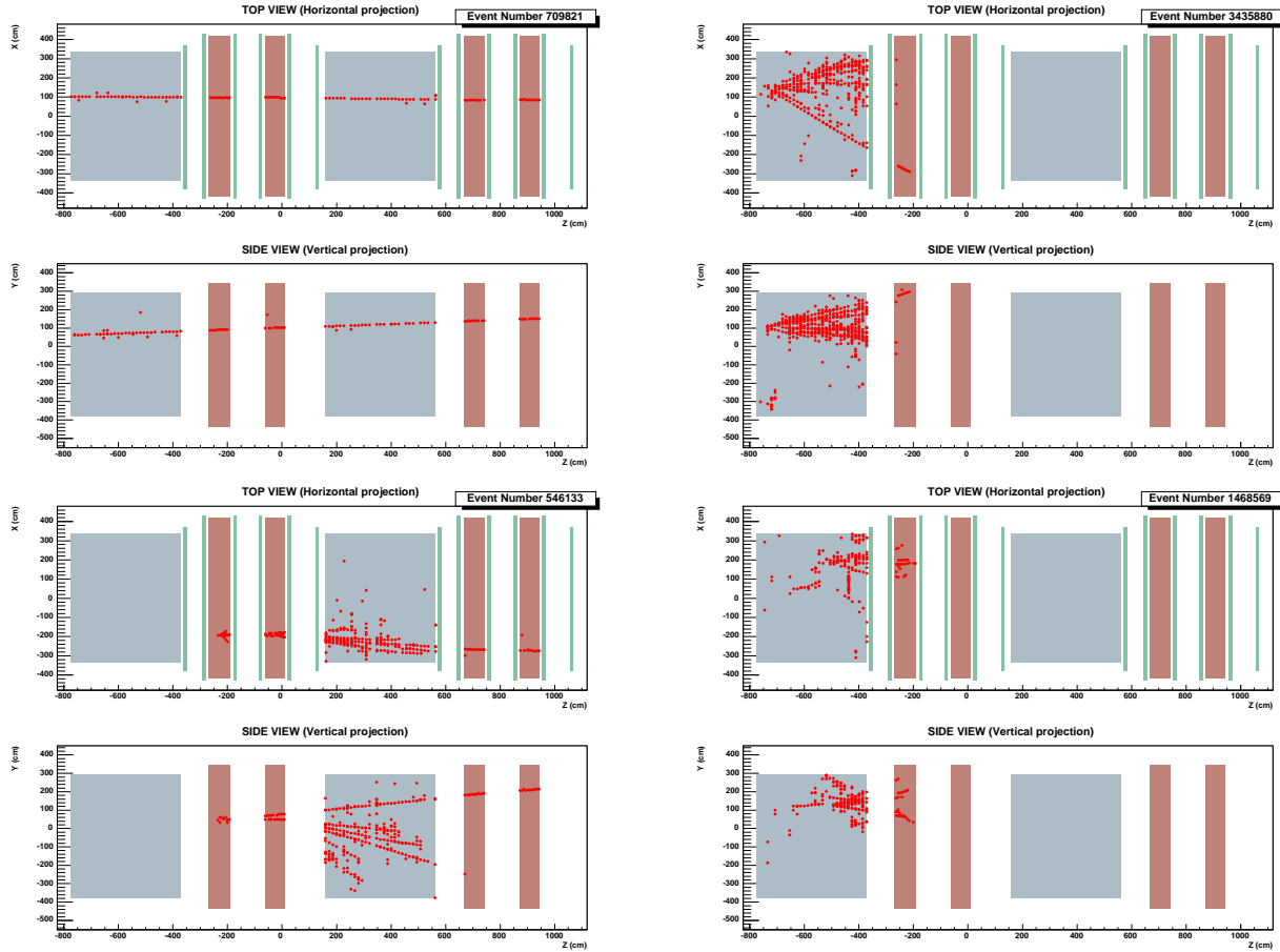
Figure 5: Display of neutrino events from the CNGS run. For each event the top and side views are shown, respectively. The SM targets are indicated in blue, the spectrometers in light brown, TT and RPC hits in red. See the text for event classification.
