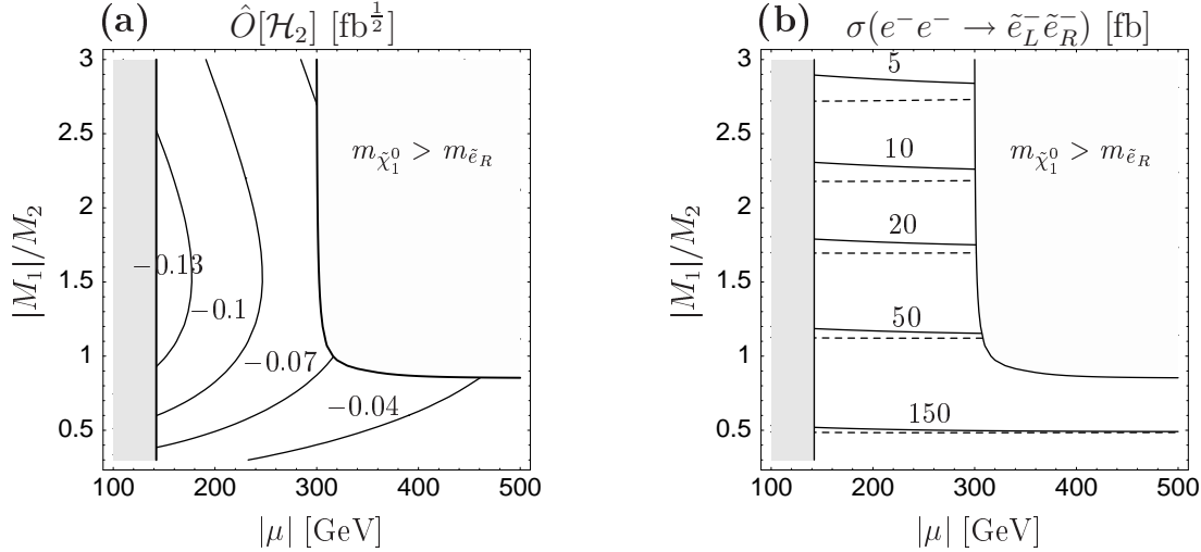
Figure 5: Contour lines (a) of the effective CP observable \hat{O}[\mathcal{H}_2] for \phi_{M_1} = 0.5\pi and (b) of the corresponding cross section \sigma(e^-e^- \rightarrow \tilde{e}_L^-\tilde{e}_R^-) for \phi_{M_1} = 0 (dashed line) and \phi_{M_1} = 0.5\pi (solid line) in the |\mu| - |M_1|/M_2 plane with M_2 = 200 GeV. The parameters which are not varied are as given in scenario A of Table 1. In the light-gray region m_{\tilde{\chi}_1^\pm} < 104 GeV and the region in the top right corner is excluded because there m_{\tilde{\chi}_1^0} > m_{\tilde{e}_R} .
