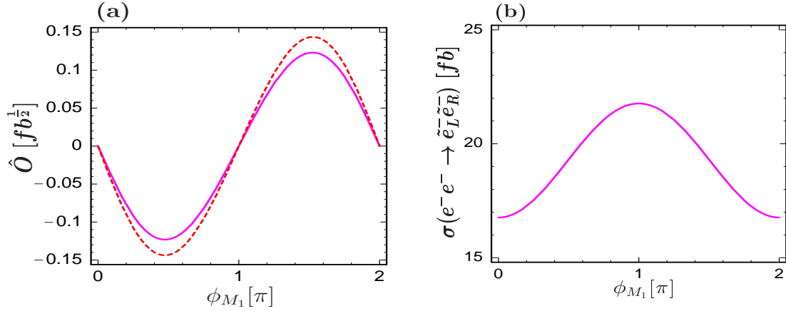
Figure 3: (a) Effective CP observable \hat{O}[\mathcal{H}_i] , Eq. (21), as a function of \phi_{M_1} for scenario B of Table 1, with \mathcal{H}_1 = \text{sign}[\cos\theta \sin(\eta - 2\phi)] (solid line) and \mathcal{H}_2 = \sin^2\theta \cos\theta \sin(\eta - 2\phi) (dashed line) and (b) the corresponding cross section \sigma(e^-e^- \rightarrow \tilde{e}_L^- \tilde{e}_R^-) .
