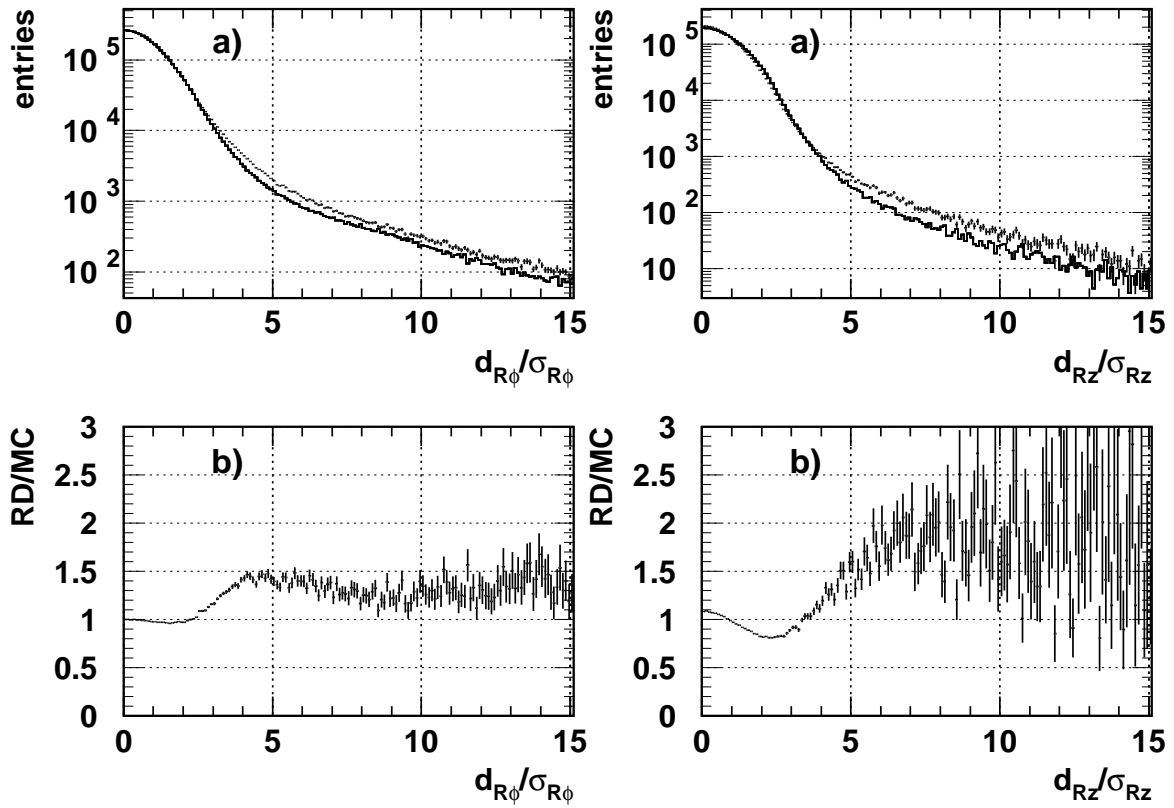
Figure 11: (a) The significance distributions for tracks with negative IP. The points with errors are real data, the histogram is simulation. (b) The ratio of these distributions (data divided by simulation). On the left for the R\phi component, on the right for Rz .
