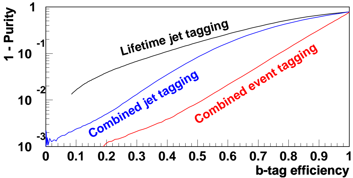
Figure 15: Background suppression in Z^0 hadronic events using combined b -tagging.
