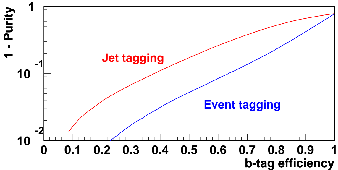
Figure 10: Background suppression in simulated Z^0 hadronic events using lifetime tagging. The efficiency is the fraction of b -jets that are tagged as coming from b -quarks, while the purity is the fraction of tagged jets that are really from b -quarks.
