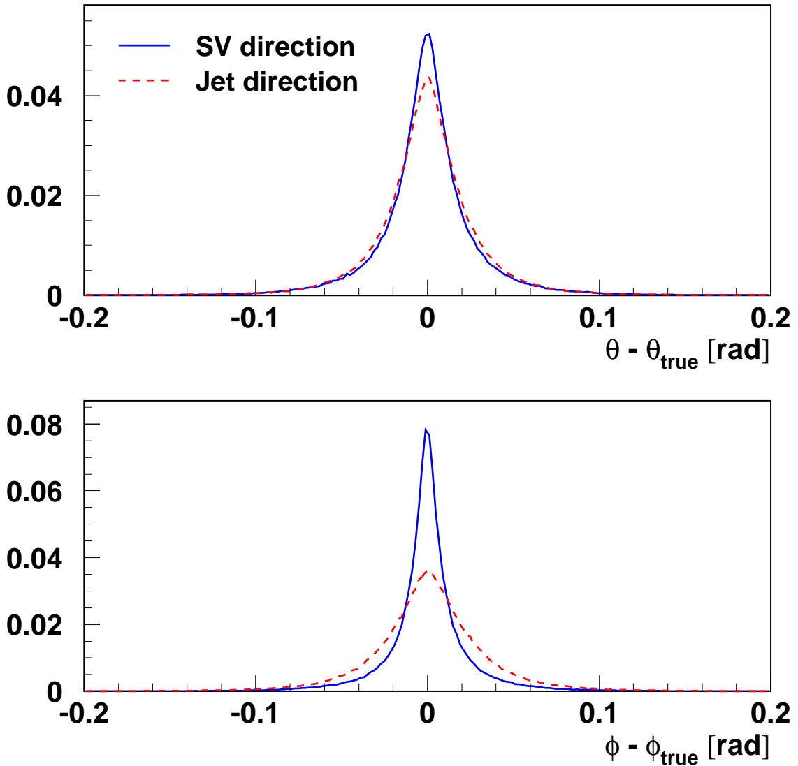
Figure 6: Distributions of the difference between reconstructed and generated directions of B hadrons for events with a reconstructed secondary vertex, for simulated Z^0 events. The B direction is defined as the direction from the primary to the secondary vertex (solid line) or as the jet direction (dashed line). Especially in \phi , the definition using the secondary vertex gives a better description of the B direction.
