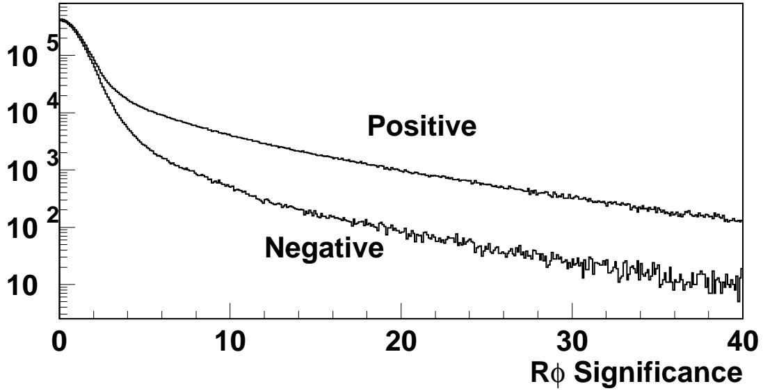
Figure 7: Distributions of positive and negative R\phi significances. The excess of tracks with large positive significance is due to long-lived particles.
