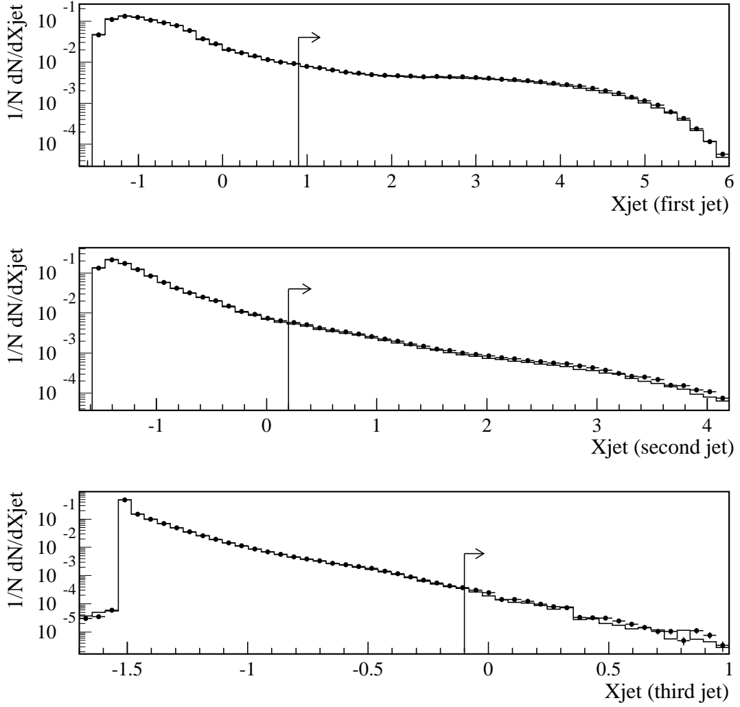
Figure 23: Distribution of the b -tagging variables for the first three jets, ordered according to their b -tagging variable, for Z^0 data (dots) and simulation (histogram). The arrows show the positions of the cuts used to select the b jets. The figure is from reference [23].
