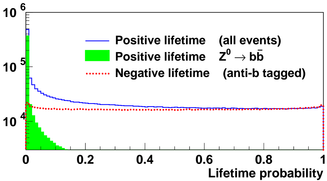
Figure 9: Distributions of positive and negative lifetime probabilities for simulated Z^0 hadronic events.
