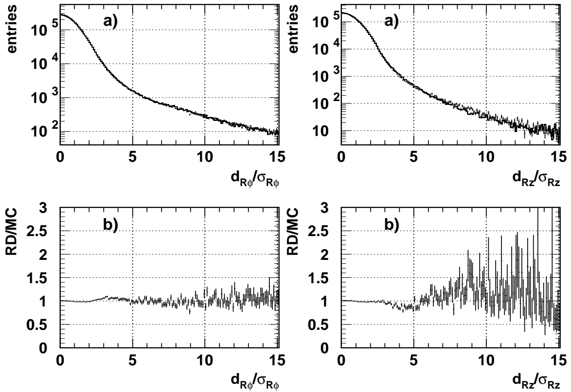
Figure 12: (a) The significance distributions for tracks with negative IP after the tuning procedure. The points with errors are real data, the histogram is simulation. (b) The ratio of these distributions (data divided by simulation). On the left for the R\phi component, on the right for Rz . These are to be compared with the corresponding distributions before tuning in fig. 11.
