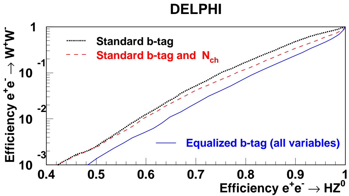
Figure 20: Mistagging efficiency for e^+e^- \rightarrow W^+W^- versus e^+e^- \rightarrow HZ^0 selection efficiency, as obtained from standard combined b -tagging, b -tagging equalised with respect to N_{ch} , and equalised b -tagging with the complete set of variables (see text for details).
