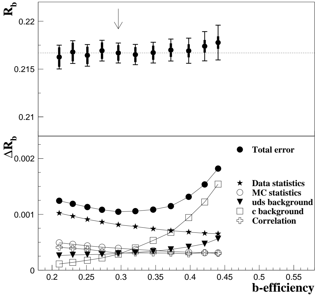
Figure 22: Stability of the R_b result as a function of the b-tagging efficiency, for data collected in 1994–5. The arrow shows the b -efficiency chosen for the final result.
