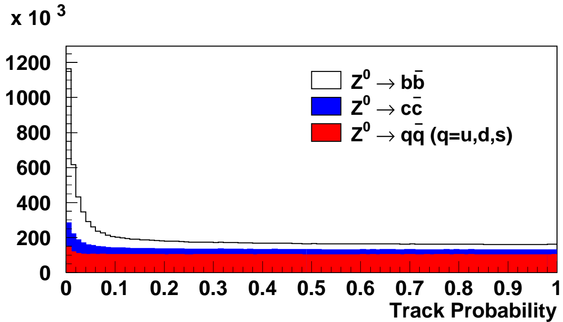
Figure 8: Simulated distributions at the Z^0 of the R\phi track IP probabilities for different quark flavours, for tracks with positive lifetime-sign IPs.
