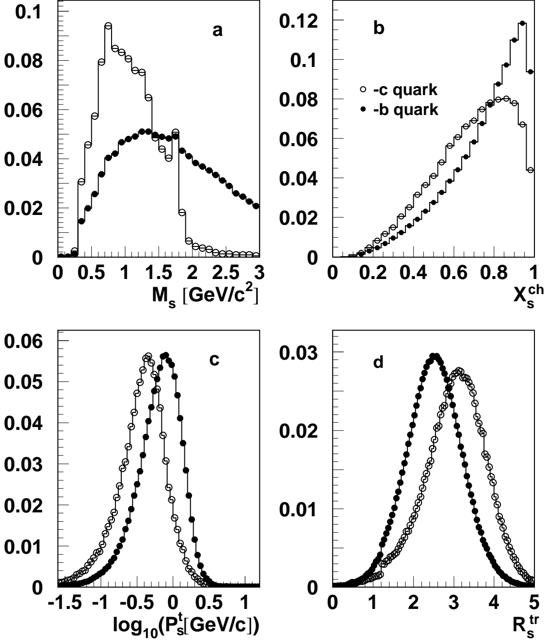
Figure 14: Distributions of discriminating variables for b - and c - quark jets for simulated Z^0 hadronic events. (a) Mass of particles in SV. (b) Fraction of charged jet energy included in SV. (c) Transverse momentum at SV. (d) Rapidity for each SV track.
