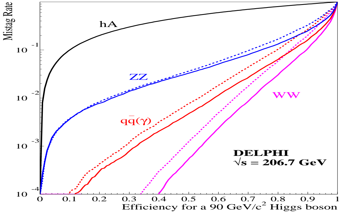
Figure 26: Expected SM background mistag rates at \sqrt{s} = 206.7 GeV, as functions of the signal efficiency for a Standard Model Higgs boson of mass 114 GeV/c 2 (top) and SUSY Higgs boson of mass 90 GeV/c 2 and \tan\beta = 20 (bottom) when varying the cut on the equalised b -tagging variable (solid lines) and combined b -tagging variable (dotted lines).
