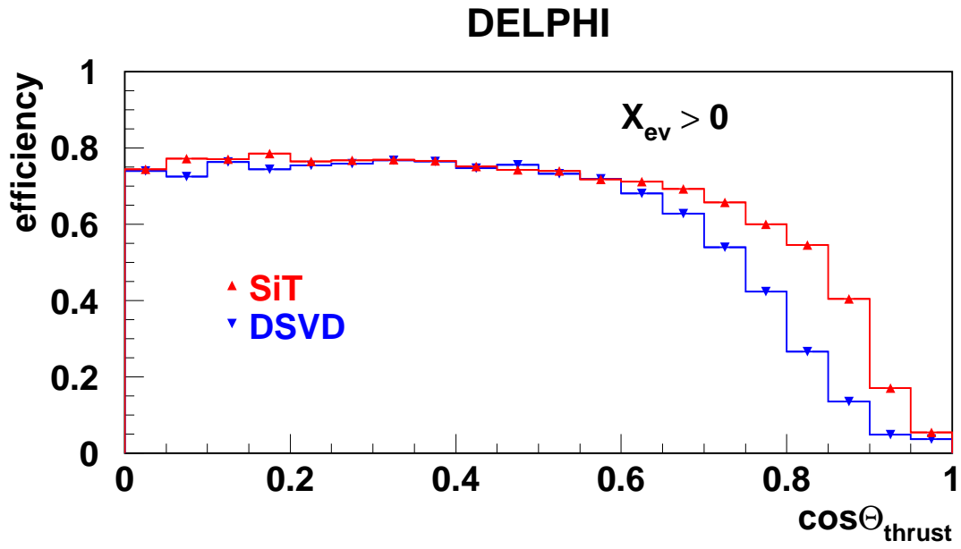
Figure 3: Selection efficiency of Z^0 \rightarrow b\bar{b} events versus \cos\theta_{thrust} using the combined event b -tagging variable X_{ev} > 0 for the SiT and the DSVD. ( X_{ev} is defined in Section 4.1.) The extra coverage provided by the SiT in the forward direction is clearly visible.
