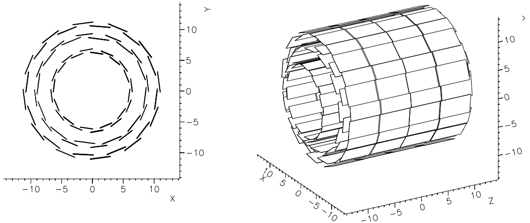
Figure 1: Schematic cross sections of the DSVD in (a) the transverse ( R\phi ) view and (b) a three-dimensional view. Dimensions are in cm.
