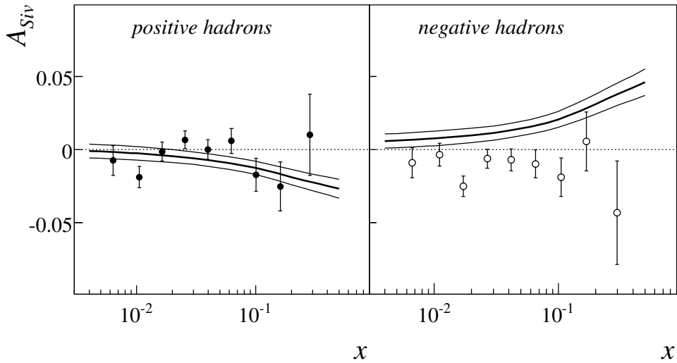
Figure 23: Comparison between the present results for positive (left) and negative (right) hadrons with the calculations of Ref. [46] (scenario 1).
