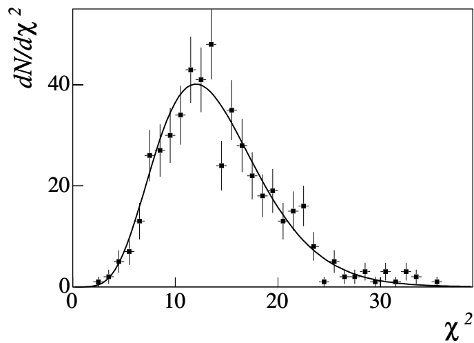
Figure 15: \chi^2 distribution of the two parameter fit used to extract the asymmetries A_j^m compared to the normalised \chi^2 distribution for ndf = 14 .
