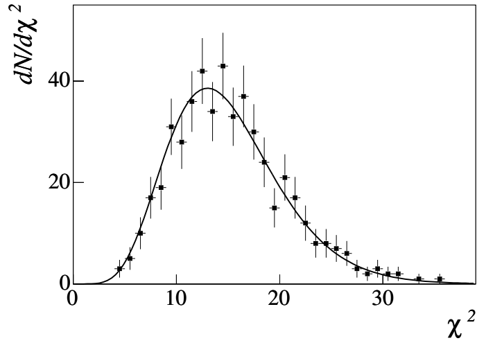
Figure 14: The \chi^2 distribution of a constant fit on R(\Phi) for the leading hadron sample compared to the normalised \chi^2 distribution for ndf = 15 .
