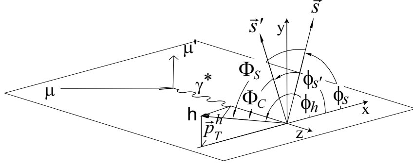
Figure 1: Definition of the Collins and Sivers angles. The vectors \vec{p}_T^h , \vec{s} and \vec{s}' are the hadron transverse momentum and spin of the initial and struck quarks respectively.
