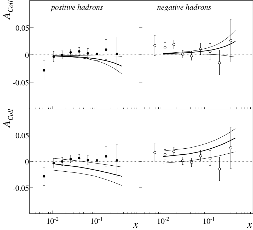
Figure 25: Comparison between the present results for positive (left) and negative (right) hadrons with the calculations of Ref. [47], where two scenarios were tested for transversity: \Delta_T q = \Delta q was assumed in one scenario (upper figures), while \Delta_T q = (q + \Delta q)/2 was assumed for the calculations of the lower figures.
