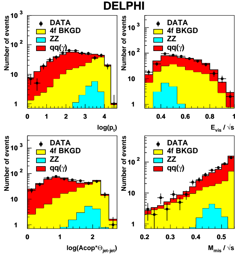
Figure 5: Distributions of four variables used in the IDA analysis stream shown after all pre-selection cuts (see text): logarithm of the transverse momentum (in GeV/c) with respect to the beam axis (upper left), ratio of the visible energy to the centre-of-mass energy (upper right), logarithm of the product of the inter-jet angle (in degrees) and the acoplanarity (lower left), ratio of the missing mass (computed using the constraint that the visible mass be compatible with M_Z ) to the centre-of-mass energy (lower right). The dots are the data taken in 1999 at a centre-of-mass energy \sqrt{s} = 199.5 GeV. The histograms are the simulation prediction.
