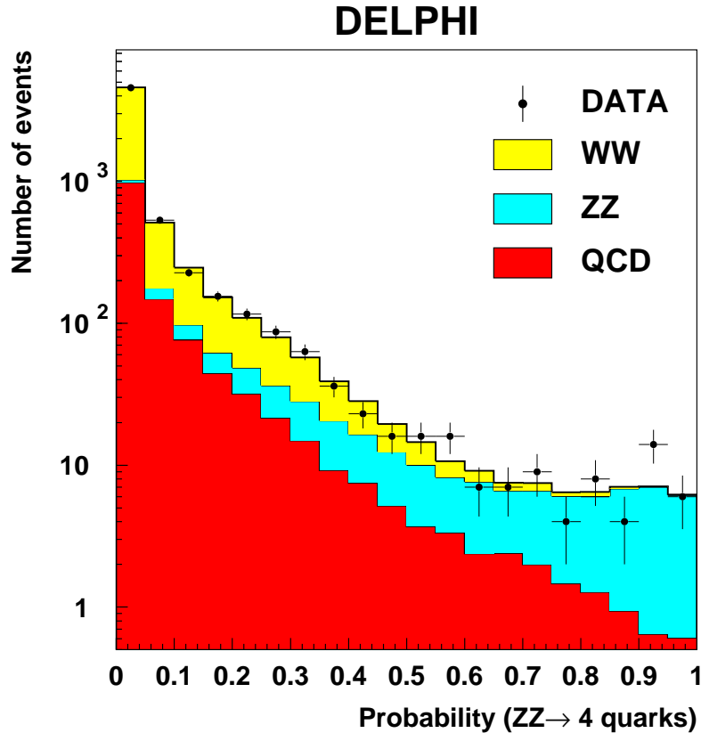
Figure 4: Distribution of the combined ZZ probability. The dots are the data taken in 1997-2000 and the histograms represent the simulation.
