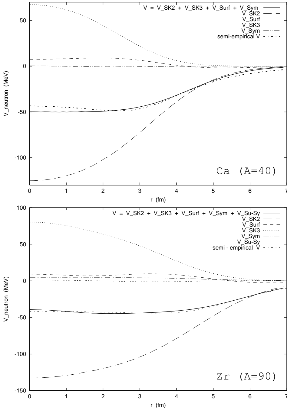
Figure 1: Radial dependence of the neutron potential for ^{40}\text{Ca} nuclei ( top ) and for ^{90}\text{Zr} nuclei ( bottom ), including the Skyrme-II attractive term (long-dashed line), the Skyrme-III repulsive term (dotted line), the symmetry term (dashed-double-dotted line) and the total (attractive + repulsive) surface term (short-dashed line). The sum of all these terms is given by the solid line and is compared to the semi-empirical central component of the neutron potential calculated according to the parameter set OB of Ref. [5] (dot-dashed line).
