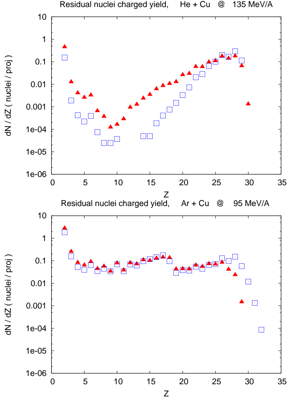
Figure 4: Residual nuclei charged yield for He + Cu at 135 MeV/A bombarding energy ( \eta = 0.88 ) ( top ) and for Ar + Cu at 95 MeV/A ( \eta = 0.22 ) ( bottom ), as predicted by QMD + FLUKA (filled triangles) and by RQMD + FLUKA (boxes).
