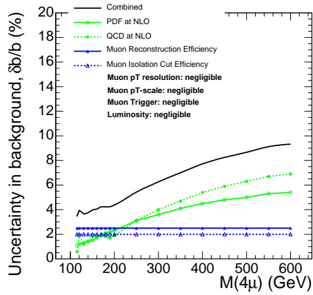
Figure 3: Uncertainties in the number of ZZ \rightarrow 4\mu background events in the signal region window at different M(4\mu) . The window size is \pm 2\sigma of the expected experimental Higgs resonance width. The event count is referenced to the number of Z \rightarrow 2\mu events. Shown are: combined uncertainty (upper solid line), PDF and QCD scale uncertainties at NLO (next two lines with circles: dashed and solid, respectively); muon reconstruction and muon cut efficiencies (two flat lines with triangles: solid and dashed, respectively).
