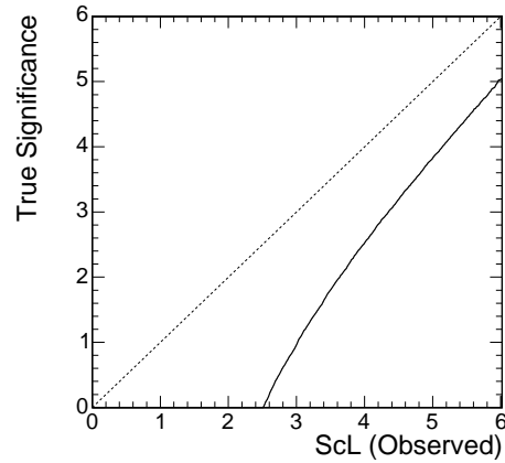
Figure 6: Local significance renormalization. Significance de-rating is required due to the fact that the search is performed in a broad range of masses.
