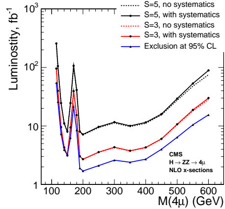
Figure 4: Integrated luminosity needed for 95%CL exclusion (triangles, lower line), 3\sigma (circles, two middle lines), and 5\sigma (circles, two upper lines) discovery versus Higgs boson mass. Dashed curves are for the case if we did not have systematic errors. Solid lines are for the case of systematic errors estimated from the measured number of Z \rightarrow 2\mu events.
