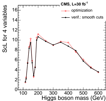
Figure 1: Significance S_{cL} vs. Higgs-boson mass: optimized cut values applied to the first half of the statistics (dashed line, empty circles) and cuts as smooth functions of 4-muon invariant mass, applied to the second half of the statistics (solid line, filled circles).
