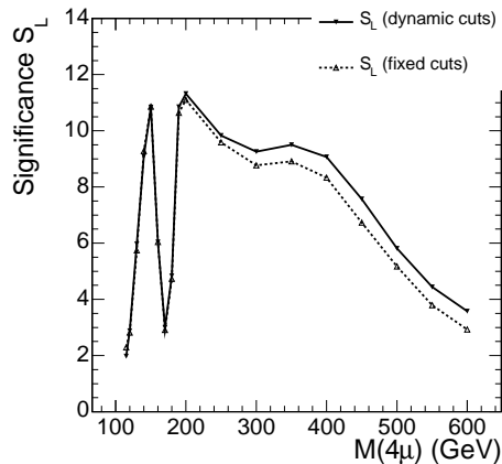
Figure 2: Expected excess significance S_L with L = 30 \text{ fb}^{-1} for different Higgs-boson masses for M(4\mu) -dependent (solid line) and independent cuts (dashed line). No systematic errors included.
