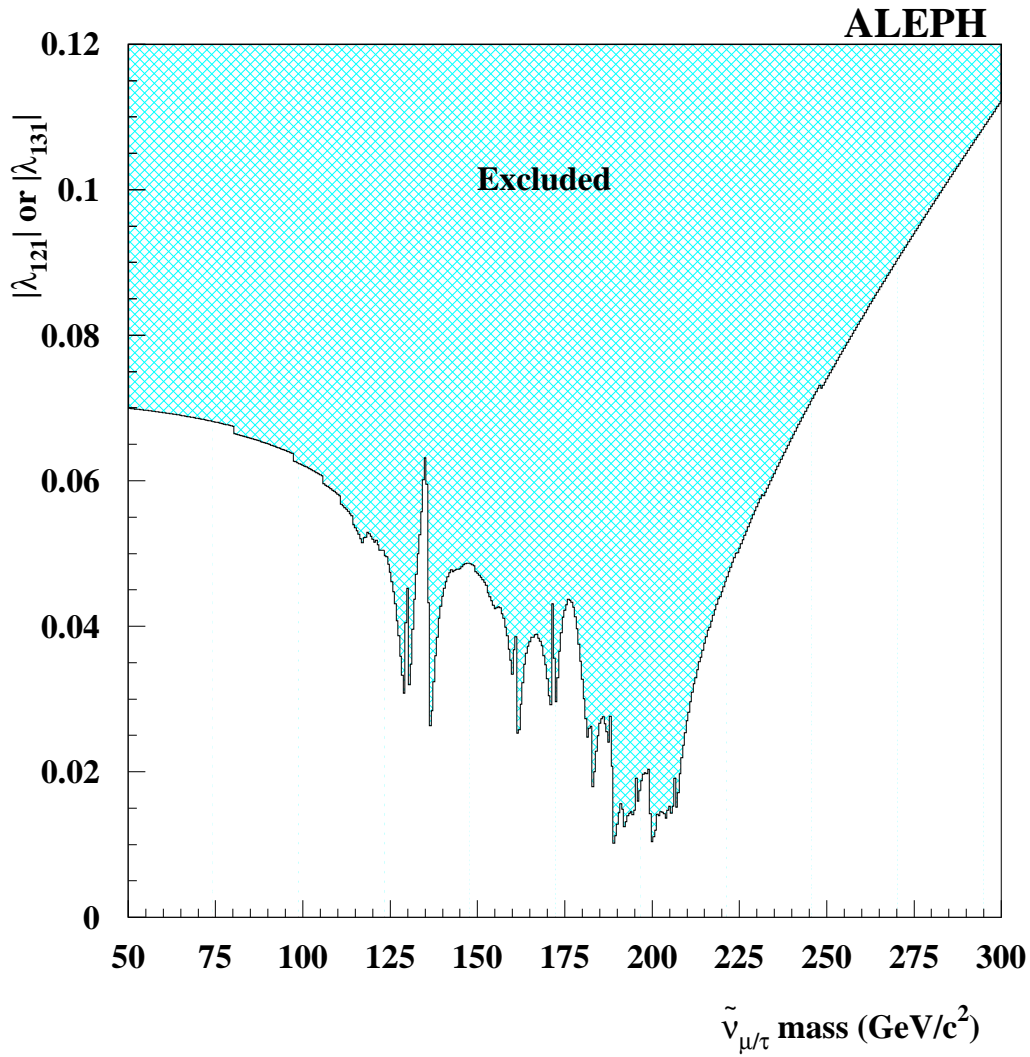
Figure 22: The 95% C.L. upper limits on the |\lambda_{121}| coupling versus the assumed \tilde{\nu}_\mu mass and on the |\lambda_{131}| coupling versus the assumed \tilde{\nu}_\tau mass, as obtained from the Bhabha cross section measurement. The \tilde{\nu}_{\mu/\tau} width is assumed to be 1 \text{ GeV}/c^2 .
