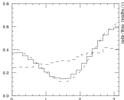
Figure 6: Normalised distribution of the azimuthal distance between the two tagging jets as in figure 5, but for Higgs + 3 parton production.
