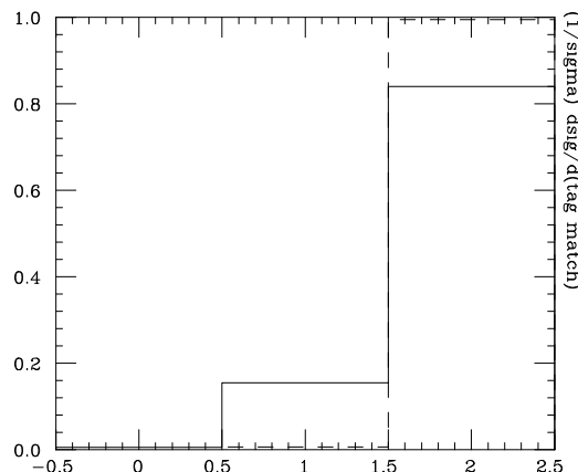
Figure 4: Same as figure 3, but for Higgs + 3 final-state-parton generated events.
