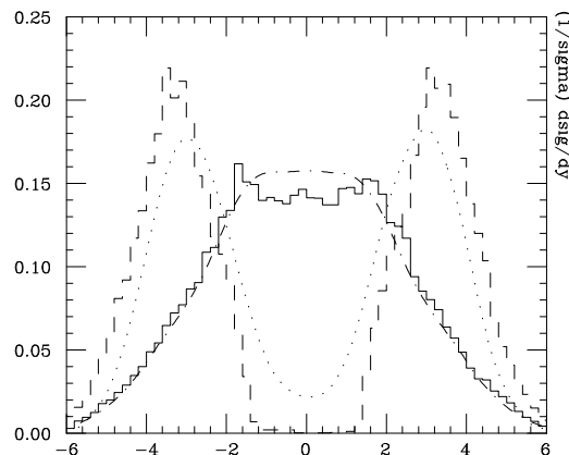
Figure 8: Normalised distribution of the rapidity of the third jet, as in figure 7, but for Higgs + 2 parton generated events after the shower.
