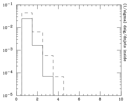
Figure 10: Normalised distribution of the multiplicity of the jets within the rapidity interval of the tagging jets, as in figure 9, but with production via VBF. Note the log scale on the vertical axis.
