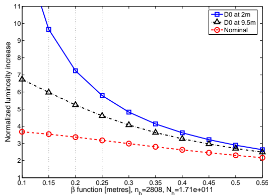
Figure 2: D0’s performance with the ultimate current.
