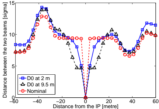
Figure 4: The separation between the two beams in the proximity of the IP 5 .
