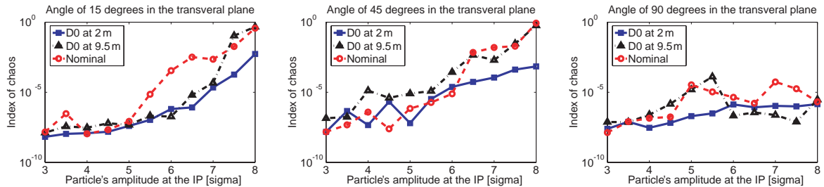
Figure 3: Analysis of the tracking results through the index of chaos, for three initial angles in the xy space.
