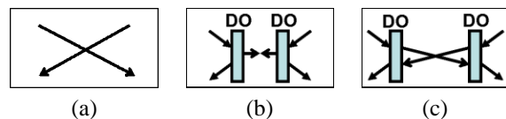
Figure 1: Crossing schemes: nominal (a), with DO at 2 m (b) and at 9.5 m (c) from the IP.
