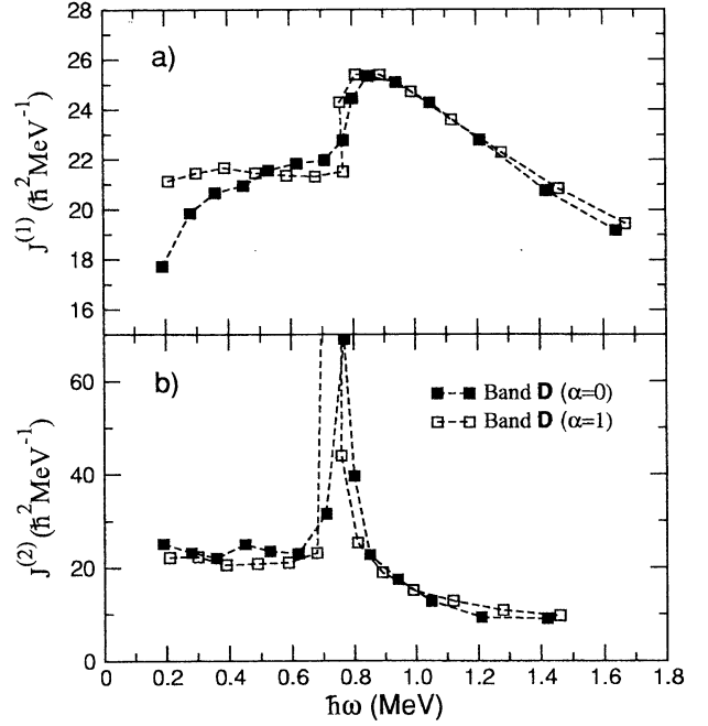
FIG. 8. (a) Kinematic and (b) dynamic moments of inertia for Band D in ^{76}\text{Kr} plotted versus rotational frequency.
