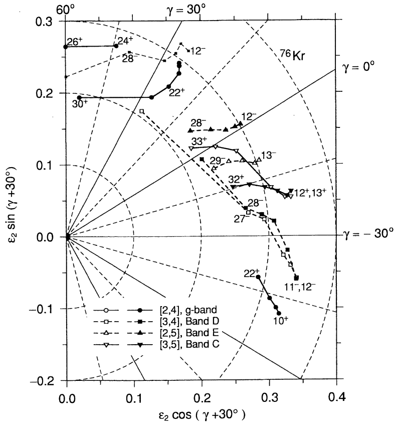
FIG. 11. Calculated deformation trajectories for ^{76}\text{Kr} . The deformations are shown for each fourth spin value except for the band terminating at I^\pi = 26^+ , where the I^\pi = 24^+ state is also shown.
