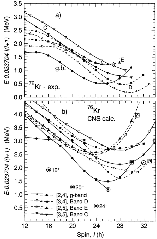
FIG. 10. Energies of high-spin collective configurations in ^{76}\text{Kr} relative to an I(I+1) reference plotted versus spin from (a) experiment and (b) configuration-dependent cranked Nilsson-Strutinsky calculations. Solid (dashed) lines represent positive (negative) parity, and closed (open) symbols denote signature \alpha = 0 ( \alpha = 1 ). In panel (b) terminating states are circled, whereas the maximum spin states that do not terminate are indicated by large squares. The calculated bands are labeled by [p, n] , where p(n) is the number of g_{9/2} protons (neutrons). The band label has been added next to the assigned configuration. A second even spin [3,4] configuration lower in energy for the spin range I \approx 25\text{--}30 is shown by a thinner line and smaller closed squares. Note that the absolute normalization for experiment and calculations is different
