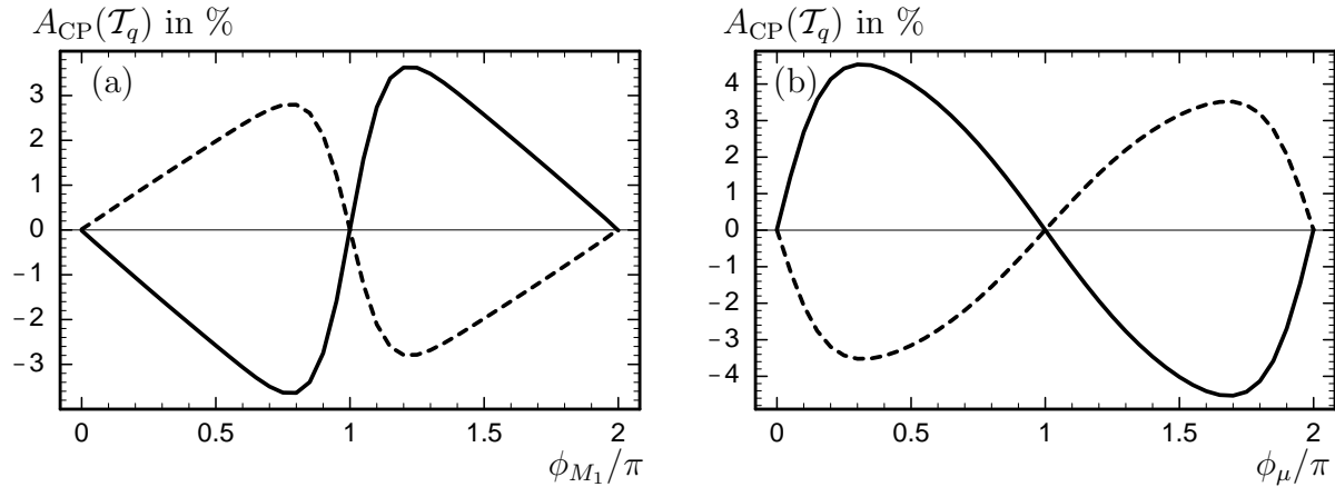
Figure 3: CP asymmetry A_{CP}(\mathcal{T}_q) , Eq. (7), for e^+e^- \rightarrow \tilde{\chi}_1^+ \tilde{\chi}_1^- with subsequent decay \tilde{\chi}_1^+ \rightarrow \tilde{\chi}_1^0 s \bar{c} for the parameters defined in Table 1 (a) with \phi_\mu = 0 and (b) with \phi_{M_1} = \pi , for \sqrt{s} = 500 GeV and for the beam polarizations (P_{e^-}, P_{e^+}) = (-0.8, +0.6) (solid), (P_{e^-}, P_{e^+}) = (+0.8, -0.6) (dashed).
