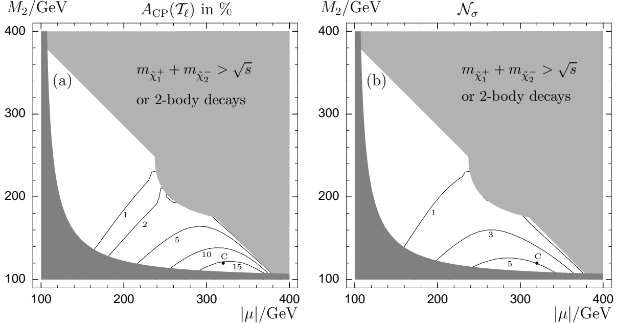
Figure 8: (a) Contours of the CP asymmetry A_{\text{CP}}(\mathcal{T}_\ell) , Eq. (7), in % for e^+e^- \rightarrow \tilde{\chi}_1^+ \tilde{\chi}_2^- at \sqrt{s} = 500 GeV with subsequent decay \tilde{\chi}_1^+ \rightarrow \tilde{\chi}_1^0 \ell^+ \nu and (b) contours of the number of standard deviations \mathcal{N}_\sigma , Eq. (18), for an integrated luminosity \mathcal{L}_{\text{int}} = 500 \text{ fb}^{-1} , respectively. The parameters are \tan\beta = 5 , m_{\tilde{\nu}} = 250 GeV, m_{\tilde{\ell}} = 261.7 GeV, |M_1|/M_2 = 5/3 \tan^2 \theta_W , \phi_{M_1} = 0 , \phi_\mu = 0.5\pi and the beam polarizations are (P_{e^-}, P_{e^+}) = (-0.8, +0.6) . The point marks the scenario C, defined in Table 3. In the dark-shaded area is m_{\tilde{\chi}_1^\pm} < 103.5 GeV, excluded by LEP [28]. The light-shaded area shows the region that either is not kinematically accessible or in which the three-body decay is strongly suppressed because m_{\tilde{\chi}_1^+} > m_W + m_{\tilde{\chi}_1^0} .
