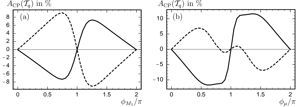
Figure 5: CP asymmetry A_{\text{CP}}(\mathcal{T}_q) , Eq. (7), for e^+e^- \rightarrow \tilde{\chi}_1^+ \tilde{\chi}_2^- with subsequent decay \tilde{\chi}_1^+ \rightarrow \tilde{\chi}_1^0 \bar{s}c for the parameters given in Table 2 (a) with \phi_\mu = 0 and (b) with \phi_{M_1} = 0 , for \sqrt{s} = 500 GeV and for the beam polarizations (P_{e^-}, P_{e^+}) = (-0.8, +0.6) (solid), (P_{e^-}, P_{e^+}) = (+0.8, -0.6) (dashed).
