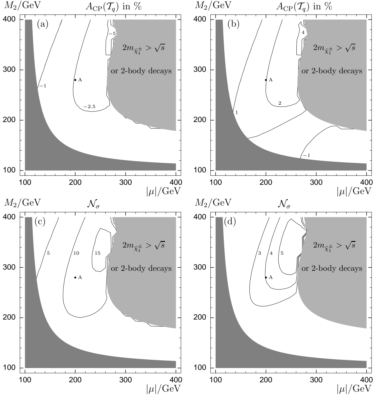
Figure 4: (a), (b) Contours of the CP asymmetry A_{\text{CP}}(\mathcal{T}_q) , Eq. (7), in % for e^+e^- \rightarrow \tilde{\chi}_1^+ \tilde{\chi}_1^- at \sqrt{s} = 500 GeV with subsequent decay \tilde{\chi}_1^+ \rightarrow \tilde{\chi}_1^0 \bar{s}c and (c), (d) contours of the number of standard deviations \mathcal{N}_\sigma , Eq. (18), for an integrated luminosity \mathcal{L}_{\text{int}} = 500 \text{ fb}^{-1} , respectively. The parameters are \tan\beta = 5 , m_{\tilde{\nu}} = 250 GeV, m_{\tilde{c}} = 500 GeV, m_{\tilde{s}} = 505.9 GeV, |M_1|/M_2 = 5/3 \tan^2\theta_W , \phi_{M_1} = 0.5\pi , \phi_\mu = 0 . The beam polarizations are in (a), (c), (P_{e^-}, P_{e^+}) = (-0.8, +0.6) and in (b), (d), (P_{e^-}, P_{e^+}) = (+0.8, -0.6) . The point marks the scenario A, defined in Table 1. In the dark-shaded area is m_{\tilde{\chi}_1^\pm} < 103.5 GeV, excluded by LEP [28]. The light-shaded area shows the region that either is kinematically not accessible or in which the three-body decay is strongly suppressed because m_{\tilde{\chi}_1^+} > m_W + m_{\tilde{\chi}_1^0} .
