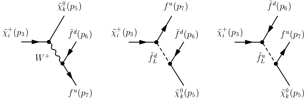
Figure 2: Feynman diagrams of the three-body decay \tilde{\chi}_i^+ \rightarrow \tilde{\chi}_k^0 \bar{f}^d f^u , where f^d = e, \mu, s and f^u = \nu_e, \nu_\mu, c .
