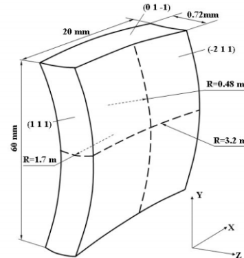
Figure 1: Bent crystal shape and atomic planes.
