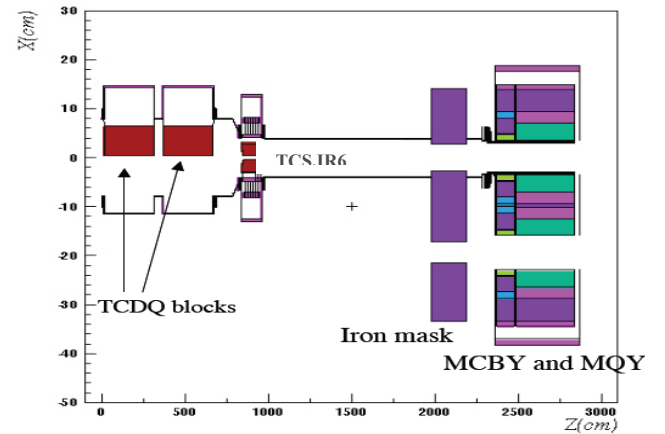
Figure 3. Horizontal section of the FLUKA geometry.
