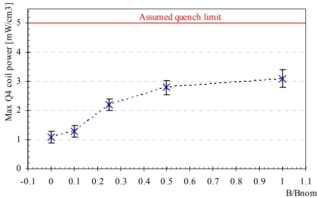
Figure 5. Sensitivity of max. power density in Q4 coil to corrector MCBY field. A factor of \sim 3 difference is seen.
