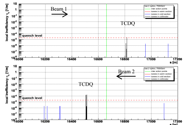
Figure 1. 7 TeV IR6 loss maps for Beams 1 and 2.
