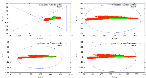
Figure 8: Beam distribution calculated with STRUCT.
