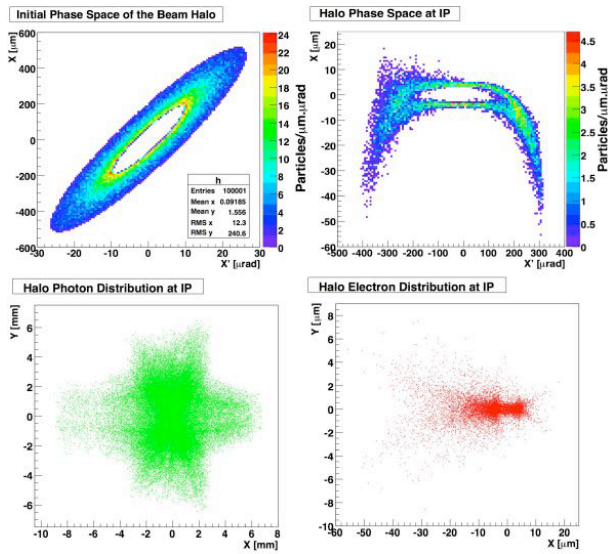
Figure 3: Top left: initial beam halo phase space. Top right: beam halo phase space at the IP. Bottom left: photon spatial distribution at the IP. Bottom right: halo electron spatial distribution at the IP.
