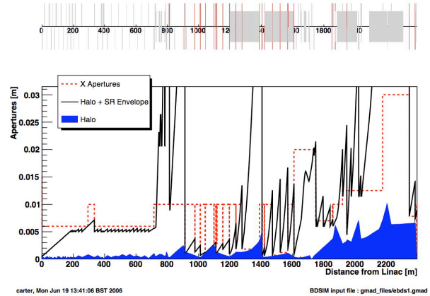
Figure 5: Beam envelope of the halo (shaded region) and the SR (solid line) in the 20 mrad BDS. Horizontal aperture of elements is also plotted (dashed line).
