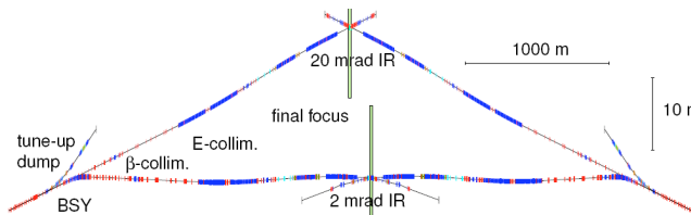
Figure 1: The layout of the ILC beam delivery system.
