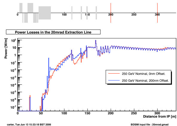
Figure 6: Normalised power losses along the 20 mrad extraction line from disrupted beam and SR. Total integrated power of 1.68 W for 0 nm and 1.66 w for 200 nm.
