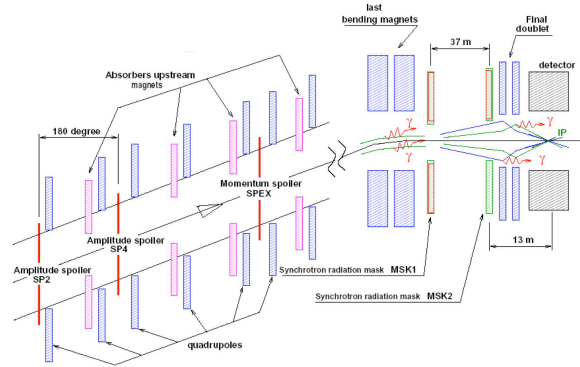
Figure 2: Sketch of ILC collimation system.
