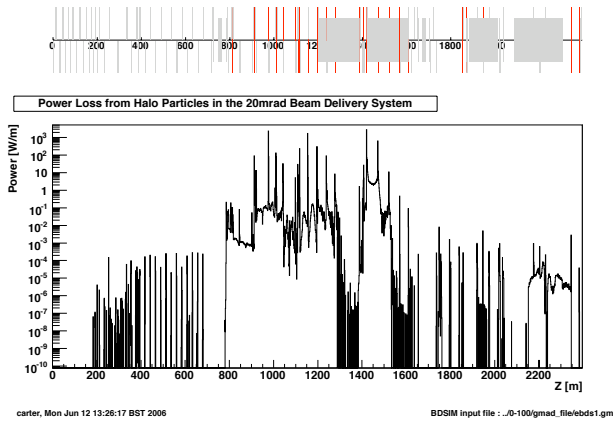
Figure 4: Normalised power losses due to beam halo and corresponding SR along the 20 mrad BDS. Given as a function of distance from the linac.
