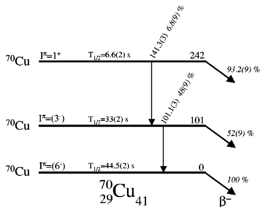
FIG. 4. The deduced relative placement for the ^{70}\text{Cu} isomers and their decay properties. The branching ratios for the isomeric transitions contain an internal conversion correction [42].
