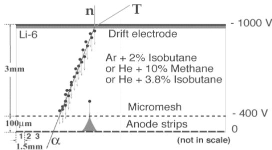
Fig. 3. The principle of Micromegas for neutron detector used in n_{\text{TOF}} experiment [8].
