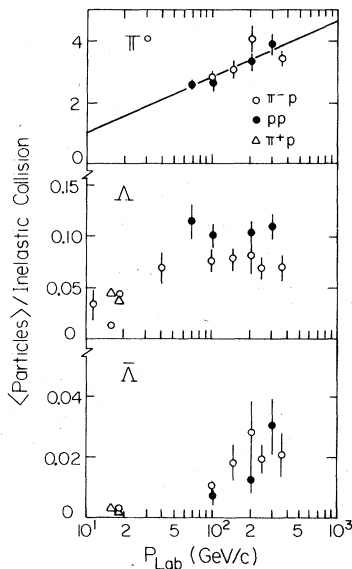
FIG. 5. Energy dependence of multiplicity of \pi^0 , \Lambda , and \bar{\Lambda} particles in \pi^-p , pp , and \pi^+p collisions. The straight line in the \pi^0 plot is from Whitmore (Ref. 5).
