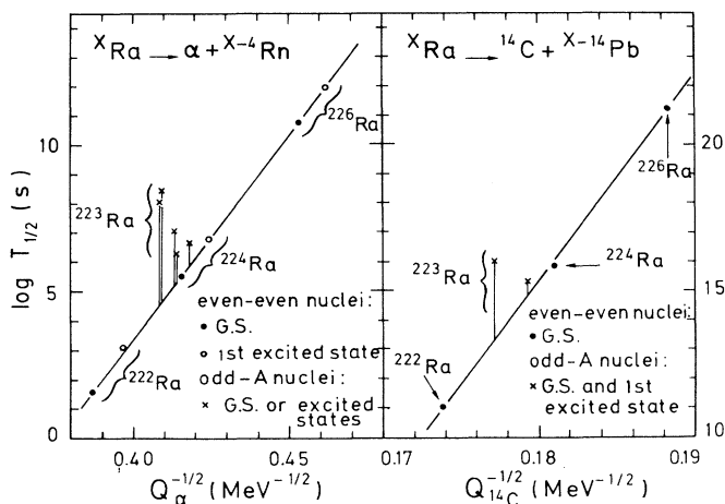
FIG. 1. Geiger-Nuttall diagram for \alpha and ^{14}\text{C} emissions of Ra isotopes. The decimal logarithm of the half-lives expressed in seconds is plotted vs Q^{-1/2} , the energy balance Q of the reaction being expressed in MeV.
