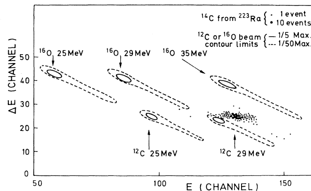
FIG. 11. The E \times \Delta E bidimensional spectrum obtained with the ^{223}\text{Ra} source. The dots represent the detected events. The contour plots represent the response of the telescope to ^{12}\text{C} and ^{16}\text{O} beams of various energies delivered by the Orsay Tandem. As expected, the event location is very close to the 29-MeV C beam. The small shift in energy has an electronic attenuation origin due to longer cables used in the measurement with beam. The E \times \Delta E = \text{const} slope, either in the measurement with the source or in the one with the beams, is due to channeling in the \Delta E detector.
