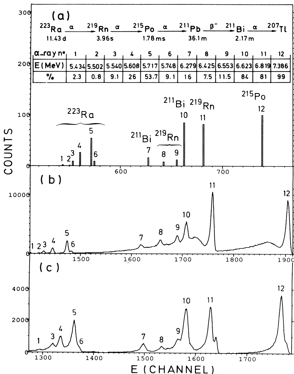
FIG. 3. The \alpha -particle spectra of the ^{223}\text{Ra} source produced at ISOLDE. In (a), the decay chain of ^{223}\text{Ra} , with the plot of the \alpha -ray intensities versus the \alpha energy, taken from Ref. [17]. In (b), the \alpha -ray spectrum of the ^{223}\text{Ra} source produced at ISOLDE, as given by a Si surface barrier detector placed in direct view of the source. In (c), as in (b), but after the deposit of an Al layer on the source by evaporation.
