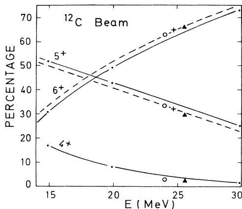
FIG. 7. The charge-state distribution plotted against the kinetic energy for ^{12}\text{C} . The continuous line connects three points taken from Ref. [18] and given for a ^{12}\text{C} beam incident on a C foil. The symbols \circ and + represent two measurements we have performed for a ^{12}\text{C} beam incident on a 100\text{-}\mu\text{g}/\text{cm}^2 Al foil. The symbol \blacktriangle represents the results of Kutschera et al. [19] for a ^{14}\text{C} beam incident on a 100\text{-}\mu\text{g}/\text{cm}^2 Al foil.
