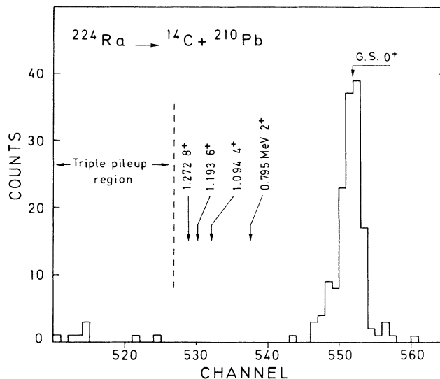
FIG. 8. The energy spectrum of ^{14}\text{C} ions measured with the ^{224}\text{Ra} source. The arrows indicate the locations of the ground state and some low-lying excited states in the residual nucleus ^{210}\text{Pb} . No events are seen at the locations of the excited states. The energy calibration has been deduced from the peak positions for the ^{223}\text{Ra} source, the latter having been calibrated in a previous experiment with a ^{14}\text{C} beam from the Tandem of Orsay. The energy resolution is 150 keV.
