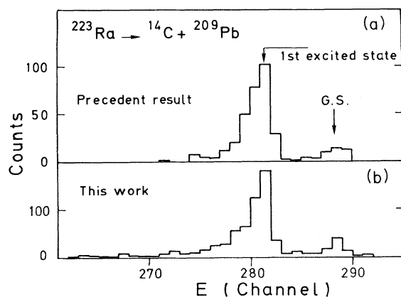
FIG. 10. Comparison of our previous result which gave evidence for the fine structure and of the present result which confirmed the discovery. The statistics in the present result are twice as high and the energy resolution is better. Low-energy tailing in both results is seen.
