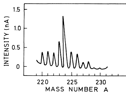
FIG. 2. The intensity of mass production at the focal chamber of ISOLDE as scanned by a wire and displayed on an oscilloscope. The peaks correspond to integer mass number A and they are composed of Fr and Ra isobars.
