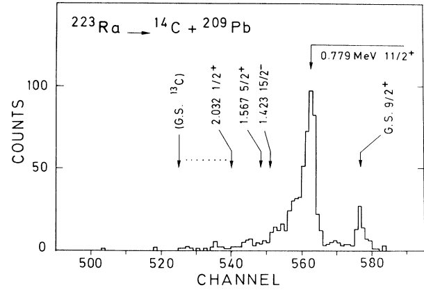
FIG. 9. The energy spectrum of ^{14}\text{C} ions measured with the ^{223}\text{Ra} source. The arrows indicate the locations of the ground state and some low-lying excited states in the residual nucleus ^{209}\text{Pb} . The presence of the peak at 0.779 MeV is the unambiguous confirmation of the evidence for a fine structure. The main parts of the ^{14}\text{C} rays show a resolution in energy of about 150 keV.
