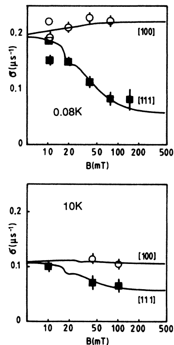
FIG. 4. Field dependence of the linewidth and fitted quadrupole interaction in Al/Ge at 0.08 and 10 K. The 0.08-K data were fitted with a pure octahedral site. The 10-K data also show an octahedral site, but not as well developed. The fit was made with 70% octahedral plus 30% tetrahedral sites.
