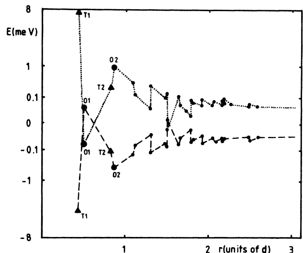
FIG. 8. The elastic energies created by the impurity at different interstitial octahedral and tetrahedral sites in Al calculated from a full expression for the interaction energies between two defects (Ref. 25). The curves are calculated for \Delta V_I = 2.9 \text{ \AA}^3 and |\Delta V_I| = 1.0 \text{ \AA}^3 . Values of \Delta V_I for different impurities are given in Table III.
