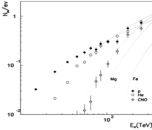
Figure 1. Number of muons per event (CORSIKA-QGSJET) reaching the MACRO depth vs primary energy. Dots from [10] and \mu energy threshold E_{\mu}^{th} = 1.6 \text{ TeV} .
