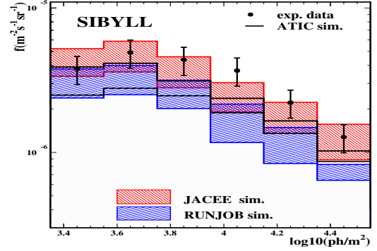
Figure 2. Measured C.I. photon density spectra (CORSIKA-SIBYLL) at distances 125 < r < 145 \text{ m} from the shower core in coincidence with \mu in MACRO. The \pm 1\sigma band expected following JACEE, RUNJOB and ATIC data is also given.
