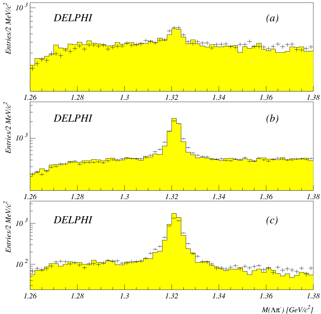
Figure 1: The right-sign ( \Lambda\pi^- and \bar{\Lambda}\pi^+ ) mass distribution with the \Xi ( \Xi^- and \bar{\Xi}^+ added) signals in different \chi^2 probability bins for data and simulation. The data are represented by the points with error bars and the simulation by the histograms, which are normalized to the same number of entries: (a) shows the \Xi signal without any other cuts applied for events with a \chi^2 fit probability below 1%, (b) shows the \Xi signal without any other cuts applied for events with a \chi^2 fit probability above 1%, (c) shows the \Xi signal after all cuts given in the text were applied for events with a \chi^2 fit probability above 1%.
