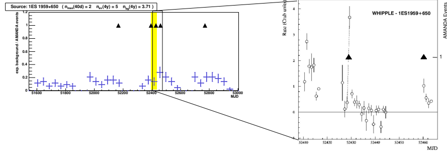
Figure 2. Left: AMANDA-II neutrino candidates within 2.25^\circ from the direction of the blazar 1ES 1959+650. The triangles indicate the arrival time of the observed events; the crosses refer to the background events in the 40-days windows. The window showing the highest multiplicity is highlighted. Right: Zoom-in of the time-window MJD 52410-52460. The arrival time of two out of the five AMANDA-II events is compared with the Whipple light curve from [5].
