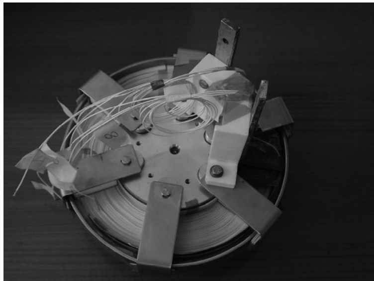
Fig. 4: Picture of an \text{MgB}_2 pancake realized with 100 meters of monocore tape.
