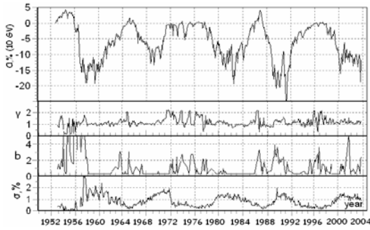
Figure 1. Parameters of galactic CR spectra variations a , \gamma and b : below – a discrepancy of the model.
