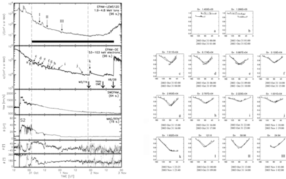
Figure 2. left: Ion, near-relativistic electron, solar wind and magnetic field observations by the EPAM, SWEPAM and MAG experiments onboard ACE during the passage of the 2 nd ICME. The black horizontal bar indicates the time interval identified by [2] as the 2 nd ICME. The dashed vertical lines indicate our identification of the ICME boundaries; right: 64-112 keV electron and 1.9-4.8 MeV ion PADs measured by the LEFS60 and LEFS150 telescopes of the EPAM instrument [3] at different times during the passage and in the vicinity of the 2 nd ICME.
