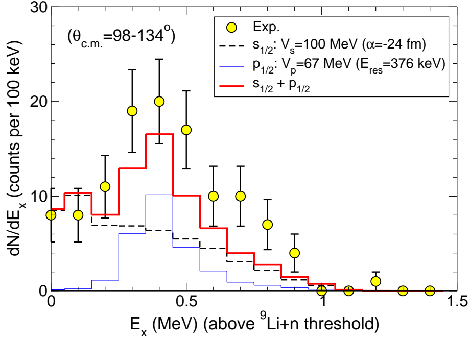
Fig. 4: (Color online) Relative contribution of s_{1/2} and p_{1/2} final states in the {}^9\text{Li}+n system to the excitation function for the reaction {}^9\text{Li}({}^2\text{H},p){}^{10}\text{Li} .
