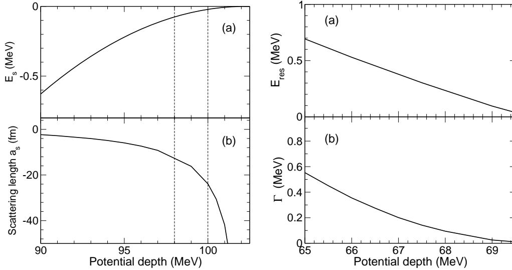
Fig. 1: Left: position (in MeV) of the s_{1/2} virtual state (upper panel) and scattering length (lower panel) as a function of the potential depth. Right: position and width of the p_{1/2} resonance as a function of the potential strength. In both cases, the {}^9\text{Li}+n potential corresponds to a Gaussian with potential radius a = 2 fm. The scattering length was calculated from the elastic phase-shift by means of the formula a_s = -\lim_{k \rightarrow 0} \tan \delta_0(k)/k . The dashed vertical lines delimit the range of values which provide acceptable fits of the measured excitation function for the s virtual state.
