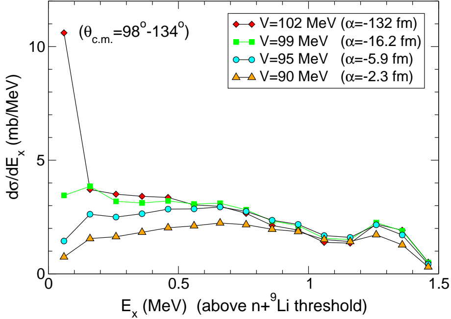
Fig. 2: (Color online) Calculated excitation function for {}^9\text{Li}({}^2\text{H},p){}^{10}\text{Li} leading to \ell = 0 states in the {}^{10}\text{Li} ( ={}^9\text{Li}+n ) system. The x-axis corresponds to the excitation energy in the {}^{10}\text{Li} system. The {}^9\text{Li}+n potential corresponds to a Gaussian with potential radius a = 2 fm, and depths indicated by the labels.
