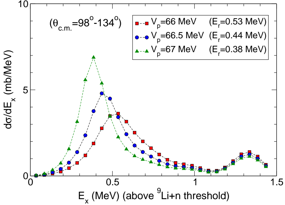
Fig. 3: Calculated excitation function for the reaction {}^9\text{Li}({}^2\text{H},p){}^{10}\text{Li} leading the \ell = 1 ( p_{1/2} ) states in the {}^{10}\text{Li} ( ={}^9\text{Li}+n ) system. The abscissas corresponds to the excitation energy in the {}^{10}\text{Li} system above the neutron- {}^9\text{Li} threshold.
