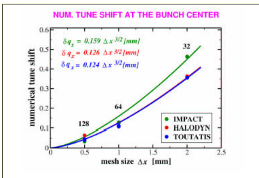
Figure JRA3.5.1: Numerical tune shift (at bunch center) generated by different codes and for three different mesh resolutions (grids with 32, 64 and 128 cells). Codes behave similar and suggest a "universal" dependence on mesh size \sim \Delta x^{3/2} .
