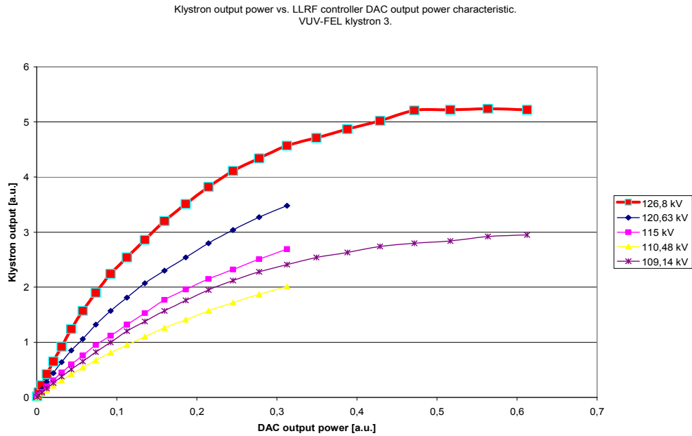
Figure JRA1.9.2: The klystron saturation phenomena in one of the VUV-FEL klystrons.
