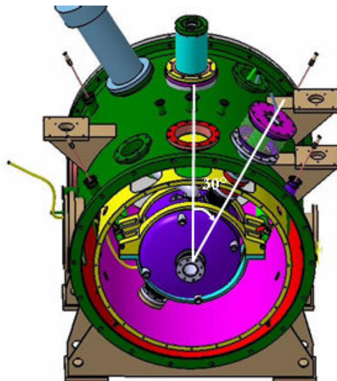
Figure JRA3.3.19: The beta 0.15 spoke cavity inside the horizontal cryostat CM0.
