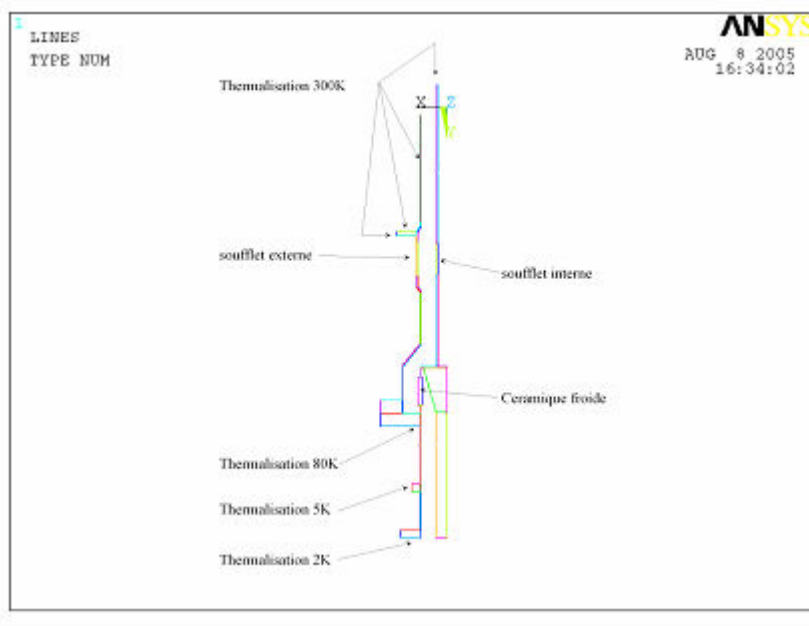
Figure JRA1.7.3: ANSYS model for the thermal calculation of TTF-V.
