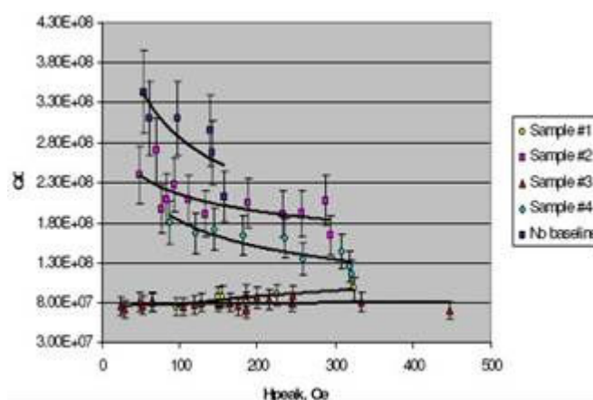
Figure JRA1.4.25: One of the \approx 10 cm diameter Nb coated Cu samples measured in Cornell (left) and measurements of the Q_0 versus H_{\text{peak}} of four such samples.
