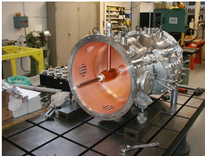
Figure JRA3.2.15: Alignment of the drift tube inside the CCDTL pre-prototype.
