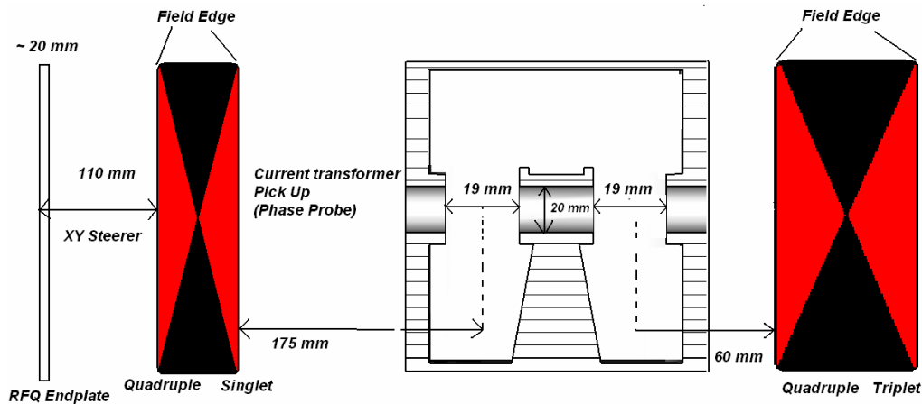
Figure JRA3.2.6: The proposed matching section between the RFQ and the first CH Tank.
