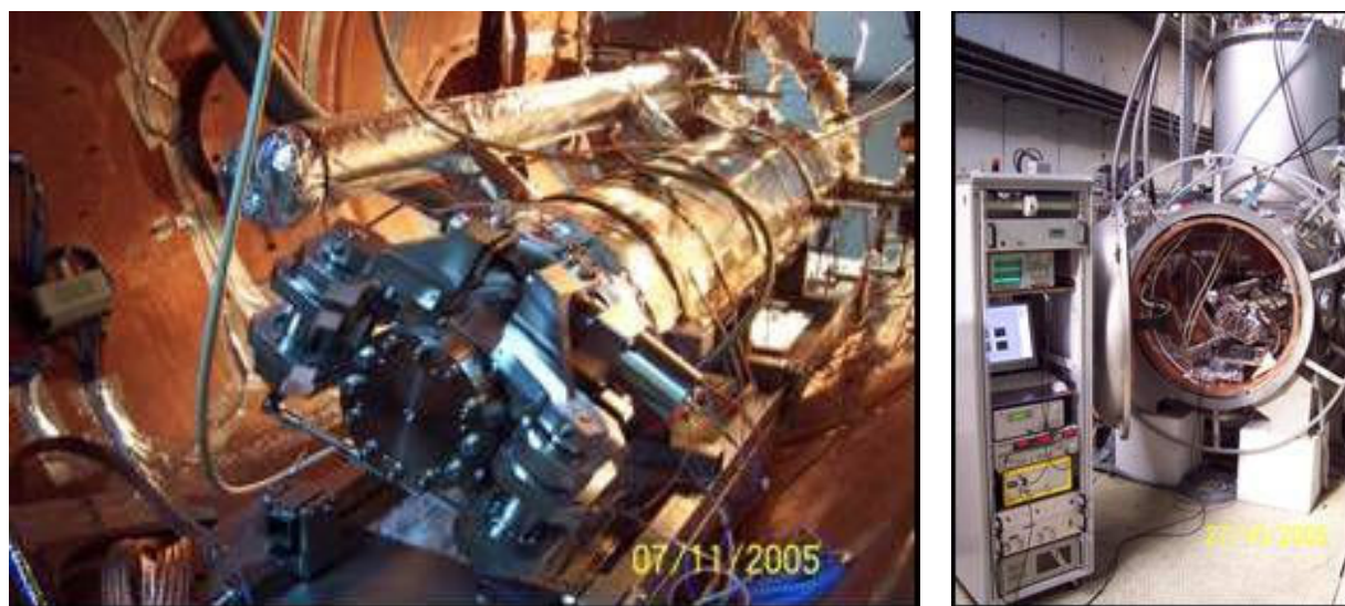
Figure JRA1.10.3: Cold Tuning System (CTS) with Noliac Piezo Tuner mounted on 9-cell cavity for cold test in CryHoLab.
