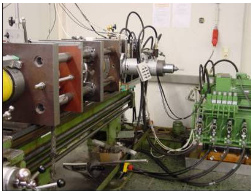
Figure JRA1.3.2: View of the tube necking machine
