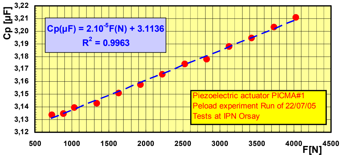
Figure JRA1.8.16. Piezoelectric actuator capacitance versus preloading force at T=4.4 K, vacuum pressure 10^{-5} mBar.
