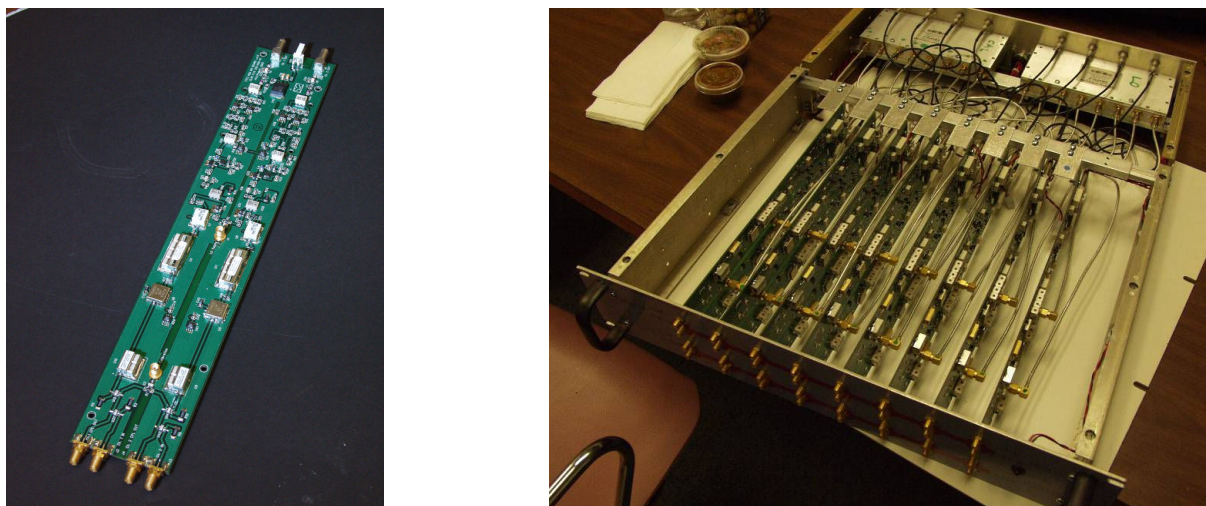
Figure JRA1.11.9: HOM electronics board for one cavity (left) and HOM electronics drawer for one TTF module of eight cavities (right), designed, built and tested at SLAC.
