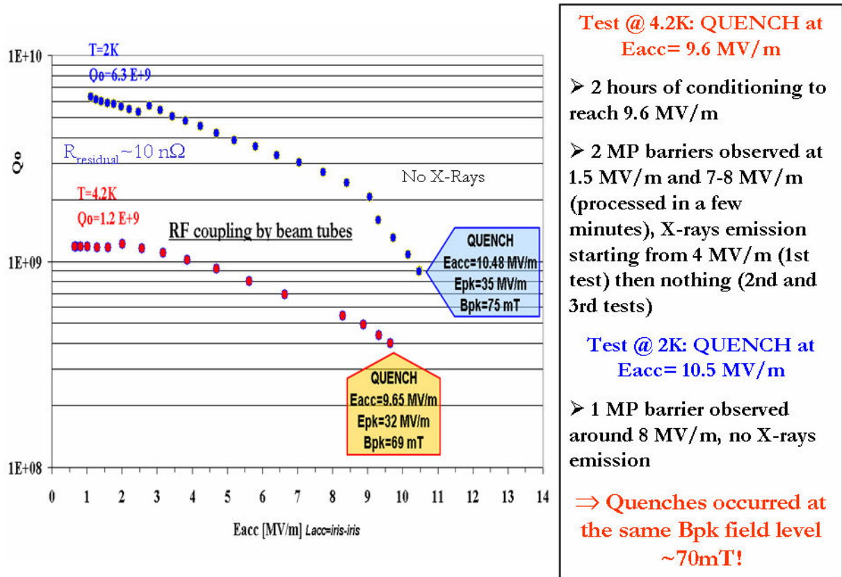
Figure JRA3.3.16: First cold tests results (2K and 4K) of the \beta_{0.15} 2-gap spoke cavity.
