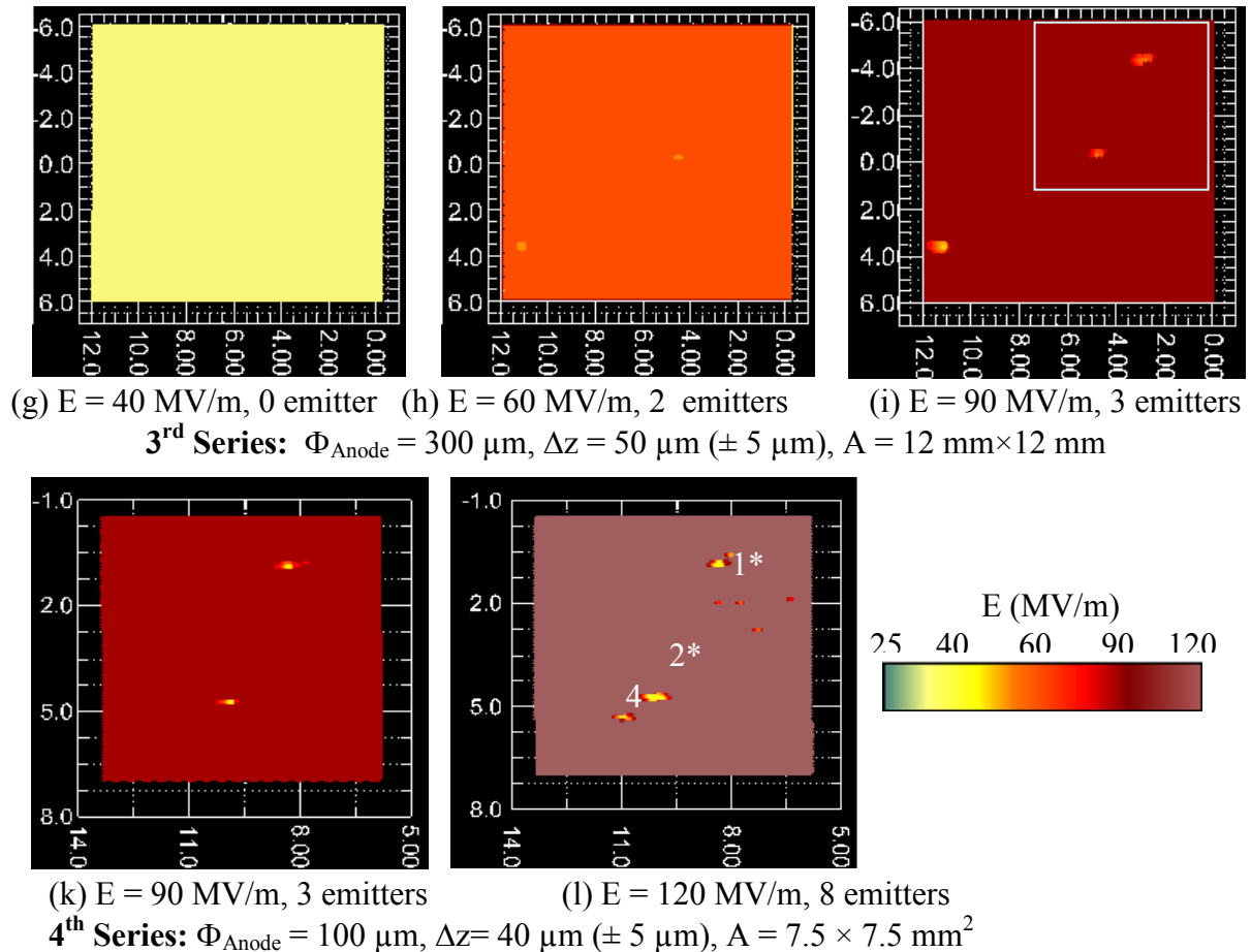
Figure JRA1.6.5: Regulated voltage maps of EP-Nb sample SEP2 after HPR at various field levels showing the onset field of emitters (color bar). The maps k and l correspond to the marked area in map i.
