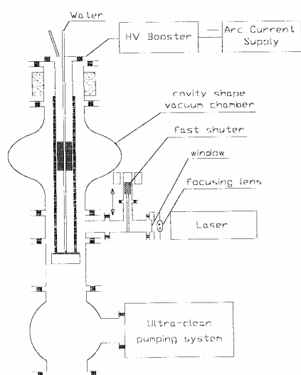
Figure JRA1.4.1: Scheme of the linear-arc UHV system and modified facility at IPJ (Swierk).
