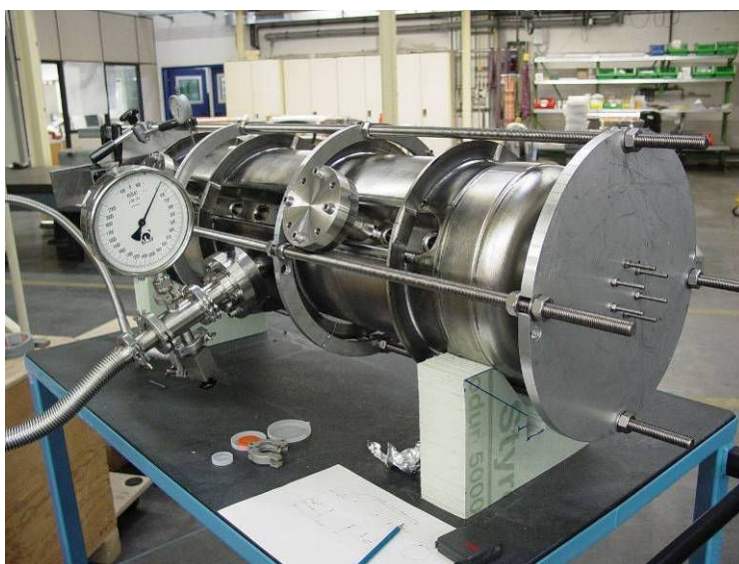
Figure JRA3.3.21: The CH-cavity during a vacuum test before the chemical treatment.
