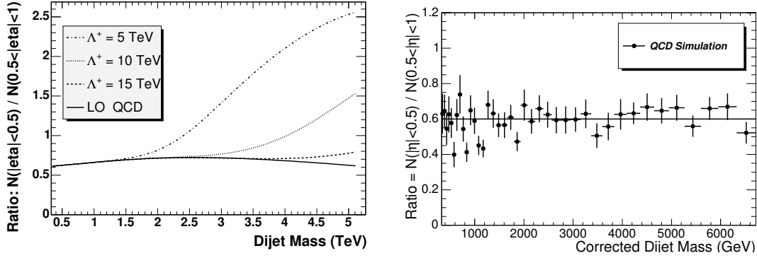
Figure 4.7: Left) A lowest order calculation of the dijet ratio from QCD (solid curve) is compared with QCD plus a quark contact interaction at a scale \Lambda^+ of 15 TeV (dashed), 10 TeV (dotted) and 5 TeV (dot-dashed). Right) The dijet ratio in the CMS simulation from QCD (points) is compared to the value 0.6 (line).
