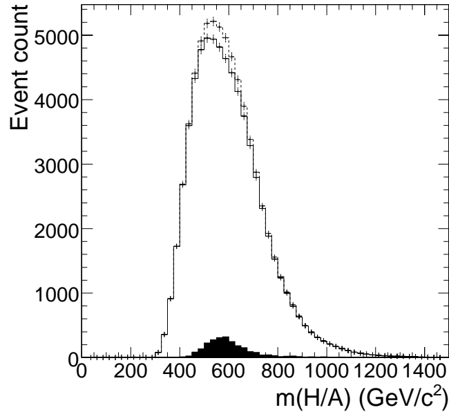
Figure 11.12: The Higgs boson mass distributions after all selections for the signal of M_A = 600 \text{ GeV}/c^2 , \tan\beta = 50 in the m_h^{\text{max}} scenario (black in foreground), background (solid line) and signal plus background (dashed line) for 60 \text{ fb}^{-1} .
