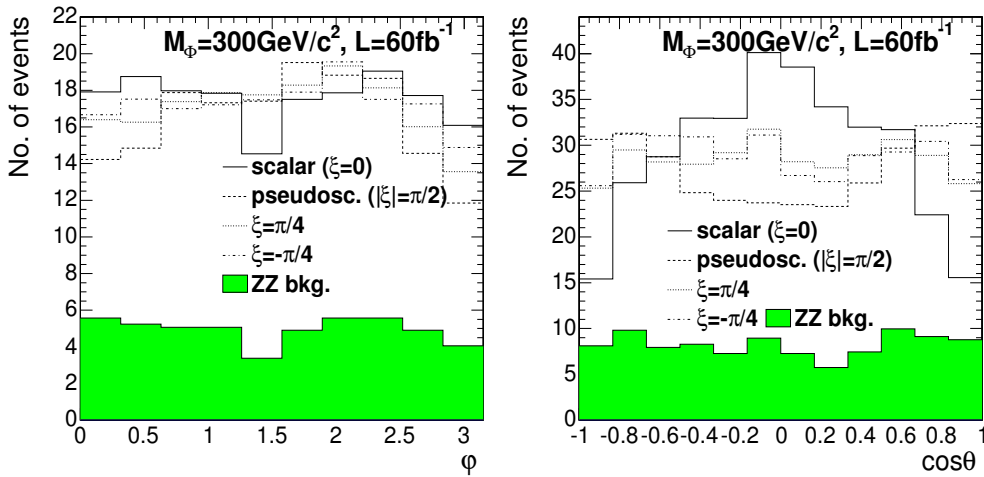
Figure 10.41: The \varphi -distributions (left) and the \theta -distributions (right) for various values of the parameter \xi after final selections at 60 \text{ fb}^{-1} . Empty histograms - the signal for M_\Phi = 300 \text{ GeV}/c^2 and \xi = 0 (scalar), \xi = -\pi/4 , \xi = +\pi/4 and |\xi| = \pi/2 (pseudoscalar). The filled histogram - the ZZ background. The Standard-Model signal cross-section and branching ratio were used for the signal normalisation.
