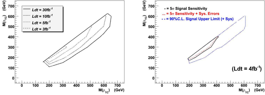
Figure 15.2: (left) Signal 5\sigma Sensitivity curves for various integrated luminosities; (right) sensitivity for \mathcal{L} = 4fb^{-1} : the dotted (resp. dashed) curve shows the sensitivity (resp. the 90% C.L. signal upper limit) after including systematic uncertainties.
