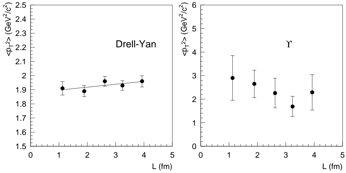
Figure 8: The L -dependence of the average transverse momentum squared for Drell-Yan dimuons in the mass range 4.5 < m_{\mu\mu} < 8 \text{ GeV}/c^2 (left plot) and for \Upsilon (right plot). For Drell-Yan, the result of a linear fit is also shown.
