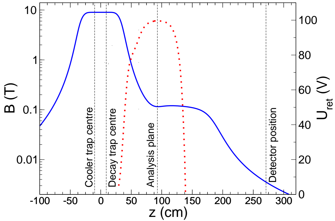
Figure 3: Magnetic field (solid line) and retardation electric field (dashed line) profile on the axis of the spectrometer ( z -axis). The retardation field has been calculated for U_{ret} = 100 V. z=0 corresponds to the center of the 9 T magnet. The positions of the traps, the analysis plane and the recoil ion detector are also indicated.
