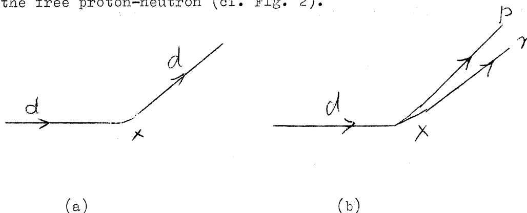
Figure 2 : An example of a two-channel reaction with non-orthogonal channels : the final states of reaction (a) are linear combinations of the final states of reaction (b).
