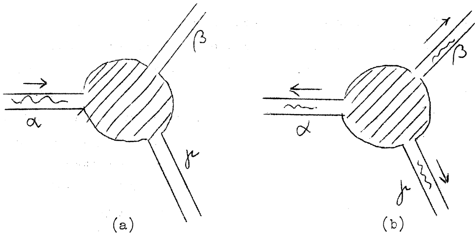
Figure 1 : Schematic representation of a three channel scattering process
