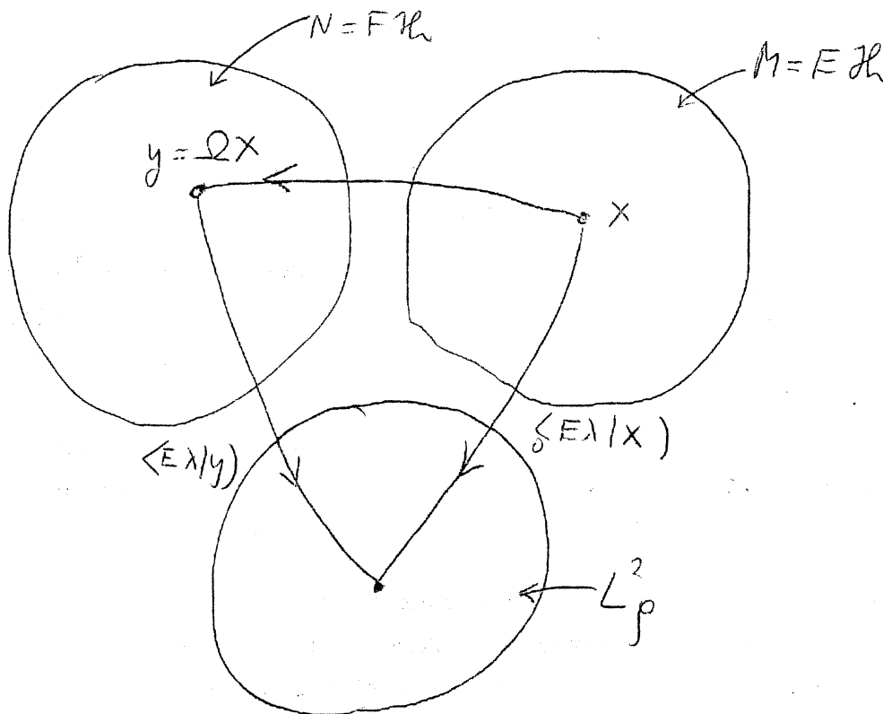
Figure 3 : Illustration of the transformation of a partial spectral representation by a partial isometry.
