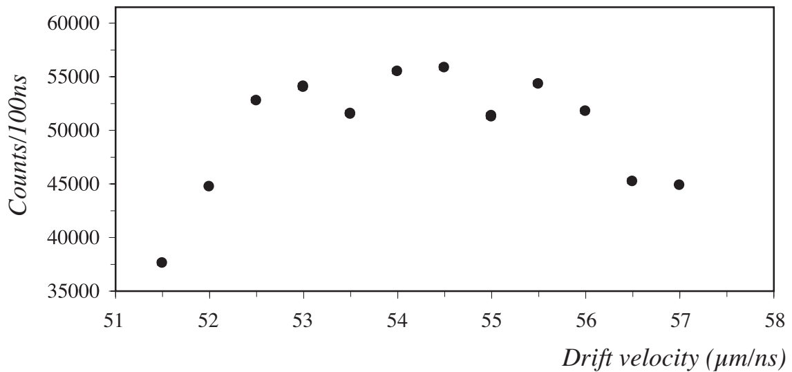
Figure 8- Autotrigger rate on a MB3 type chamber (HH and HL triggers only) for cosmuics as a function of the drift velocity settings. The regular efficiency drop every three steps is due to an hardware bug in the BTI ASIC which cannot be corrected. The hole is filled when allowing uncorrelated triggers.
