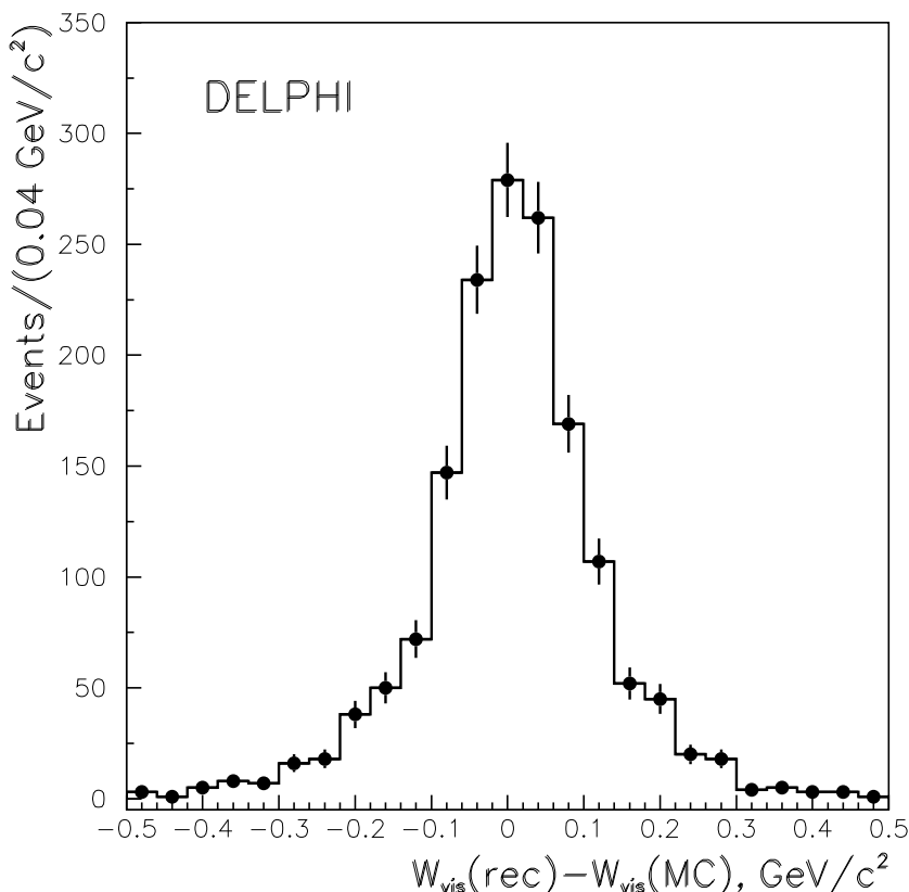
Figure 2: Difference between reconstructed and generated W_{vis} values for the selected 4 charged-particle events from the Monte Carlo \gamma\gamma \rightarrow q\bar{q} sample, in the \eta_b search region.
