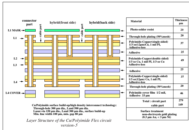
Figure 6 Layer construction of SCT barrel Cu/Polyimide flex-circuit
