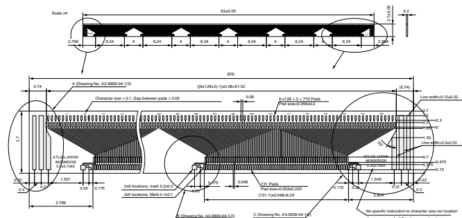
Figure 7 SCT barrel aluminium-on-glass pitch-adapter: overall (top) and enlarged sections (bottom)
