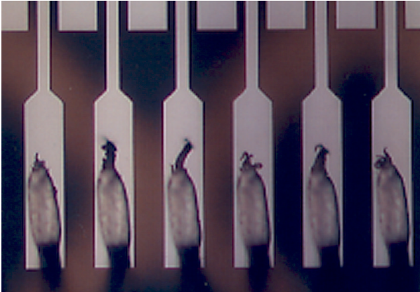
Figure 9 Typical whiskers generated in PA before improved
