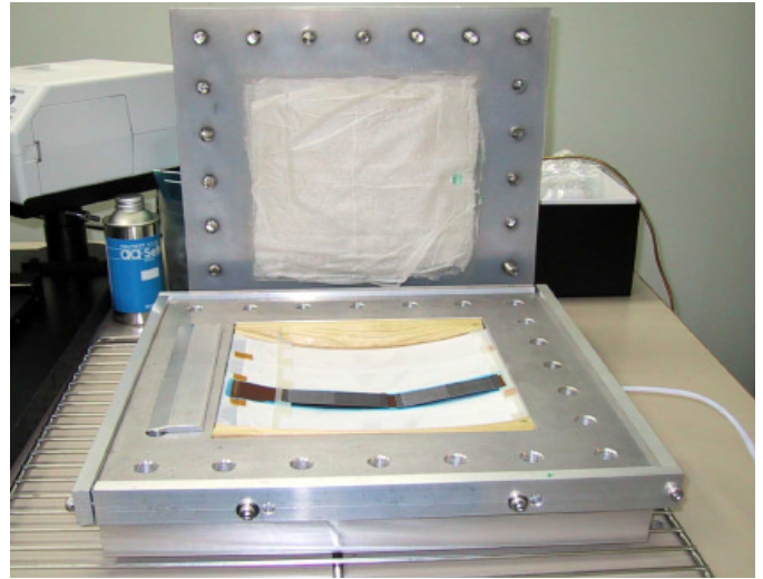
Figure 8 The heat-press jig for the SCT barrel hybrid
