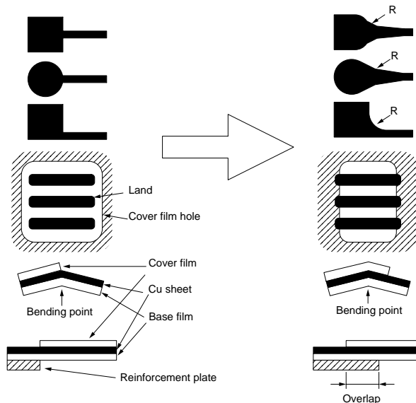
Figure 5 Cu/Polyimide flex circuit design rules from the ref. [5]
