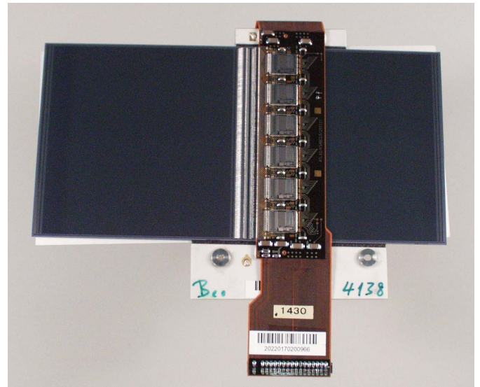
Figure 2 SCT barrel module
