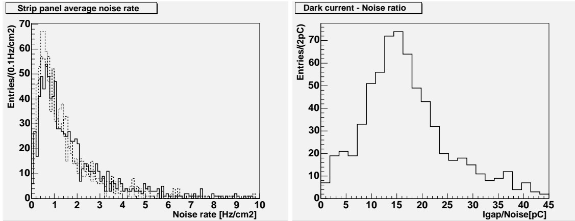
FIGURE 5. Noise rate distribution (on the left) for different high voltage values of 10kV (...), 10.1kV (-.-), and (-) 10.2 kV. Current-to-Noise ratio distribution at a high voltage value of 10kV (on the right). The data are taken from the ATLAS RPC tested in Lecce with an equivalent input voltage threshold of about 0.5 mV.
