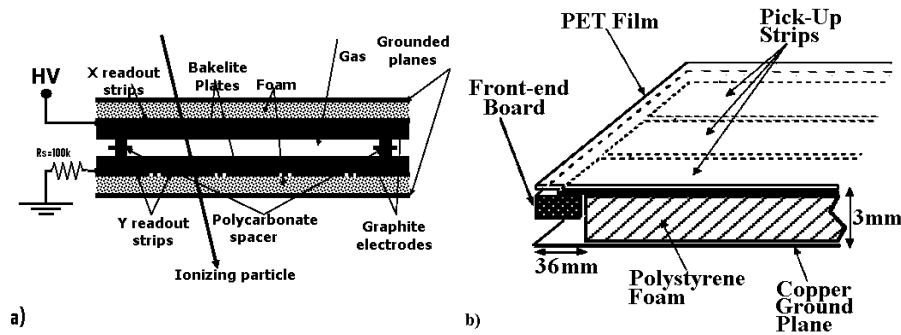
FIGURE 1. Drawing of ATLAS RPC layer (a) and read-out strip panel (b).
