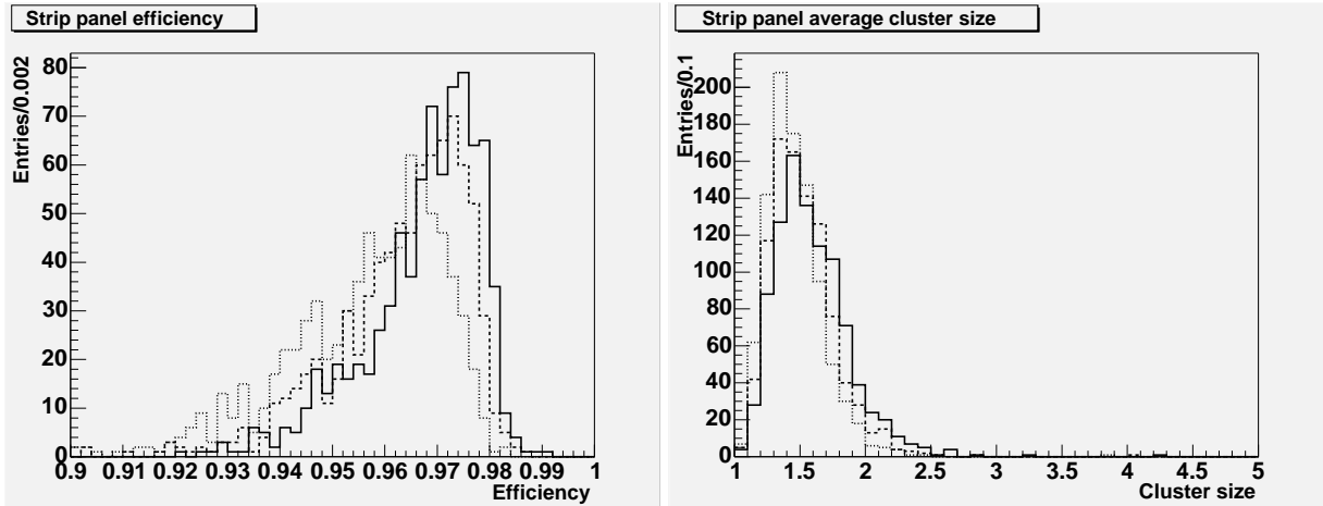
FIGURE 4. Total efficiency distribution (on the left) and average cluster size distribution (on the right) for different high voltage values of 10kV (...), 10.1kV (-.-), and (-) 10.2 kV. The data are taken from the ATLAS RPC tested in Lecce with an equivalent input voltage threshold of about 0.5 mV.
