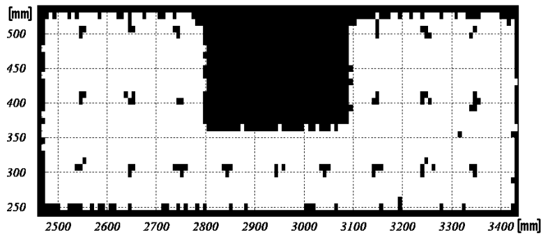
FIGURE 3. Example of tomography plot of a small size gas volume with cut-out. The dark regular spot array are due to the spacers dead area.
